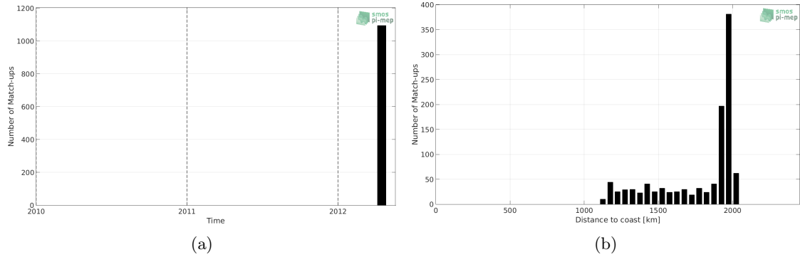
Figure 1: Number of match-ups between TSG-GOSUD-Research-vessel and CCI-L4-ESA-MERGED-OI-V1.8-30DAY-RUNNING SSS as a function of time (a) and as function of the distance to coast (b) over the SPURS 2 Pi-MEP region and for the full satellite product period.
