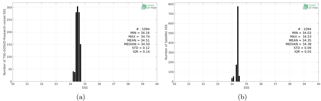
Figure 2: Histograms of SSS from TSG-GOSUD-Research-vessel (a) and CCI-L4-ESA-MERGED-OI-V1.8-30DAY-RUNNING (b) considering all match-up pairs per bins of 0.1 over the SPURS 2 Pi-MEP region and for the full satellite product period.
