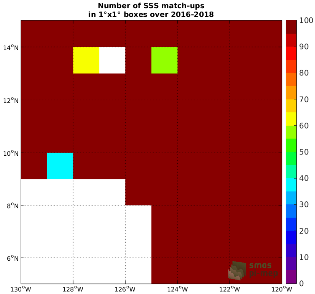
Figure 3: Number of SSS match-ups between Surface drifters SSS and the CCI L4 Merged-OI v1.8 - 30-day running (ESA) SSS product for the SPURS 2 Pi-MEP region over 1°x1° boxes and for the full satellite product period.
