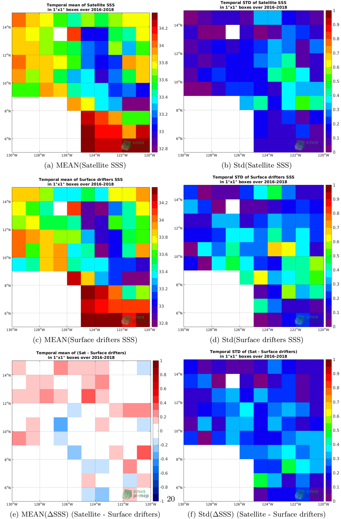
Figure 5: Temporal mean (left) and Std (right) of SSS from CCI L4 Merged-OI v1.8 - 30-day running (ESA) (top), Surface drifters (middle), and of \Delta SSS (Satellite - Surface drifters). Only match-up pairs are used to generate these maps.
