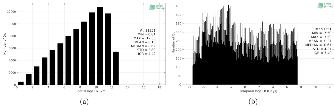
Figure 4: Histograms of the spatial (a) and temporal (b) lags between the time of the Surface drifters measurements and the date of the corresponding CCI L4 Merged-OI v1.8 - 30-day running (ESA) SSS product.
