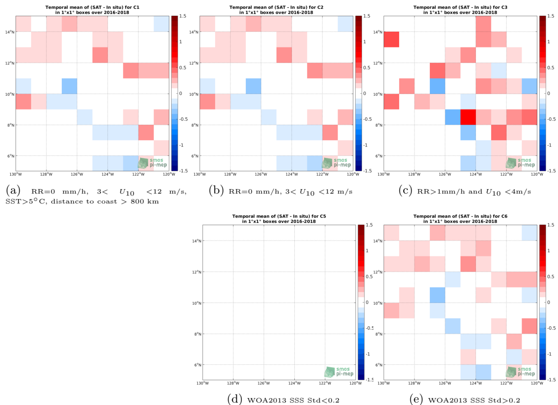
Figure 11: Temporal mean gridded over spatial boxes of size 1^\circ \times 1^\circ of \Delta SSS (CCI L4 Merged-OI v1.8 - 30-day running (ESA) - Surface drifters) for 5 different subdatasets corresponding to:RR=0 mm/h, 3 < U_{10} < 12 m/s, SST >5^\circ\text{C} , distance to coast > 800 km (a), RR=0 mm/h, 3 < U_{10} < 12 m/s (b), RR >1 mm/h and U_{10} < 4 m/s (c), WOA2013 SSS Std <0.2 (d), WOA2013 SSS Std >0.2 (e).
