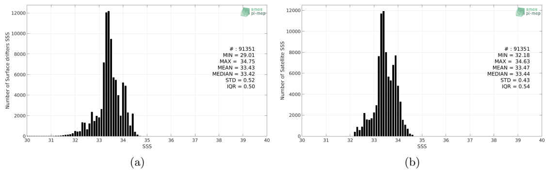
Figure 2: Histograms of SSS from Surface drifters (a) and CCI L4 Merged-OI v1.8 - 30-day running (ESA) (b) considering all match-up pairs per bins of 0.1 over the SPURS 2 Pi-MEP region and for the full satellite product period.
