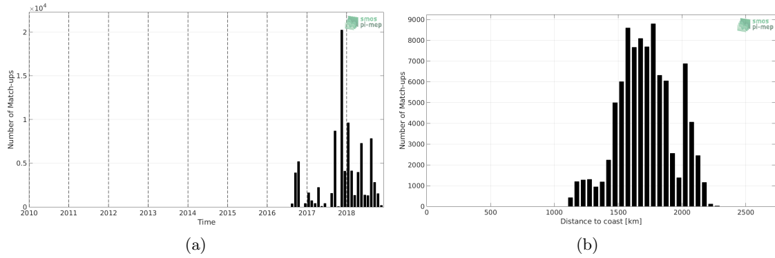
Figure 1: Number of match-ups between Surface drifters and CCI L4 Merged-OI v1.8 - 30-day running (ESA) SSS as a function of time (a) and as function of the distance to coast (b) over the SPURS 2 Pi-MEP region and for the full satellite product period.
