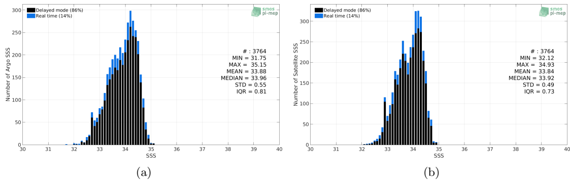
Figure 2: Histograms of SSS from Argo (a) and CCI-L4-ESA-MERGED-OI-V1.8-30DAY-RUNNING (b) considering all match-up pairs per bins of 0.1 over the SPURS 2 Pi-MEP region and for the full satellite product period.
