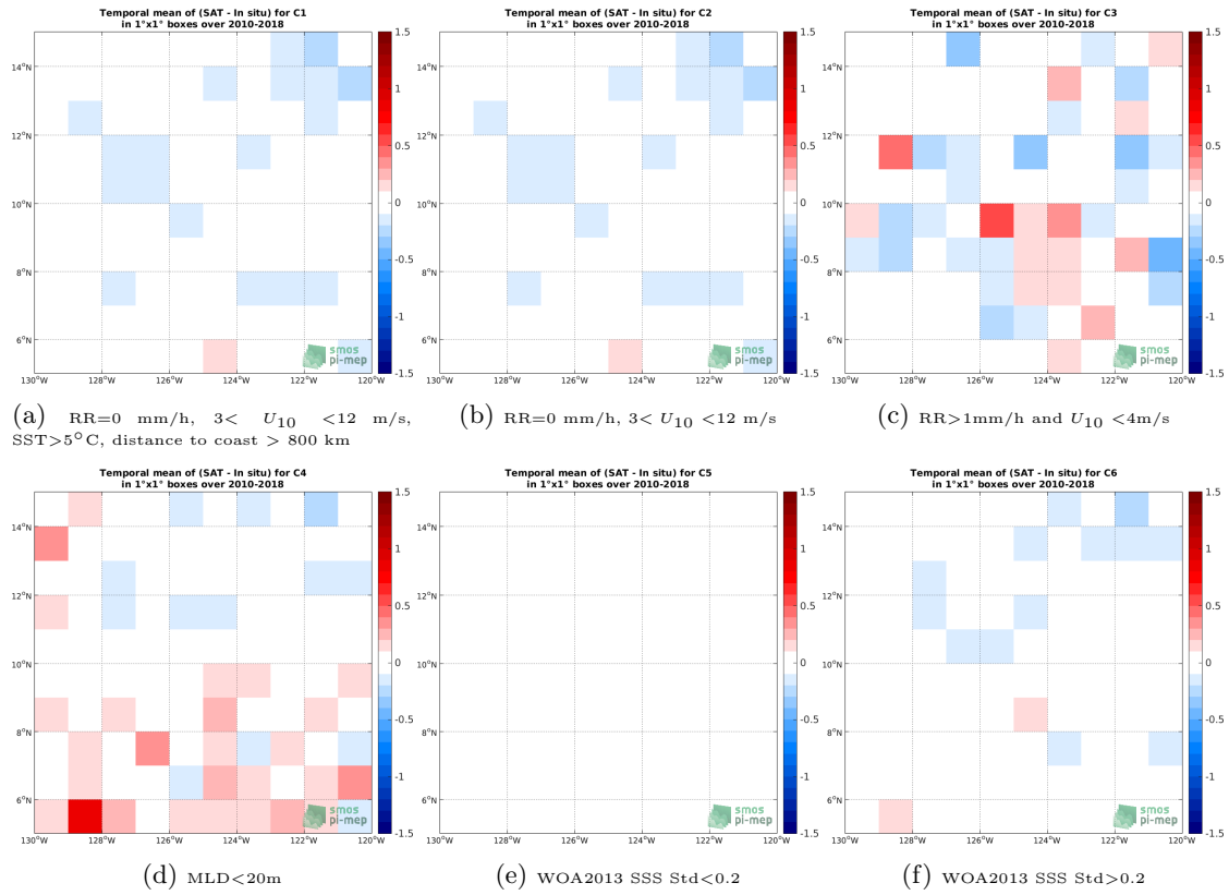
Figure 12: Temporal mean gridded over spatial boxes of size 1^\circ \times 1^\circ of \Delta SSS (CCI-L4-ESA-MERGED-OI-V1.8-30DAY-RUNNING - Argo) for 6 different subdatasets corresponding to:RR=0 mm/h, 3 < U_{10} < 12 m/s, SST >5^\circ C, distance to coast > 800 km (a), RR=0 mm/h, 3 < U_{10} < 12 m/s (b), RR >1 mm/h and U_{10} < 4 m/s (c),MLD <20 m (d),WOA2013 SSS Std <0.2 (e),WOA2013 SSS Std >0.2 (f).
