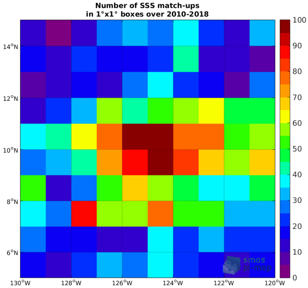
Figure 4: Number of SSS match-ups between Argo SSS and the CCI-L4-ESA-MERGED-OI-V1.8-30DAY-RUNNING SSS product for the SPURS 2 Pi-MEP region over 1°x1° boxes and for the full satellite product period.
