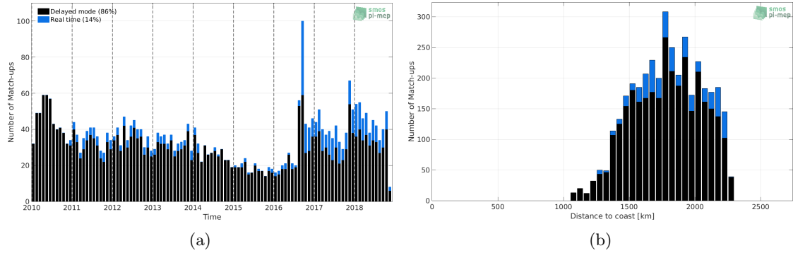
Figure 1: Number of match-ups between Argo and CCI-L4-ESA-MERGED-OI-V1.8-30DAY-RUNNING SSS as a function of time (a) and as function of the distance to coast (b) over the SPURS 2 Pi-MEP region and for the full satellite product period.
