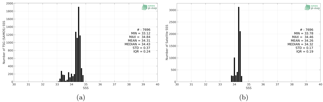
Figure 2: Histograms of SSS from TSG (SAMOS) (a) and Aquarius SSS L4 OI v5 - Weekly (IPRC) (b) considering all match-up pairs per bins of 0.1 over the SPURS 2 Pi-MEP region and for the full satellite product period.
