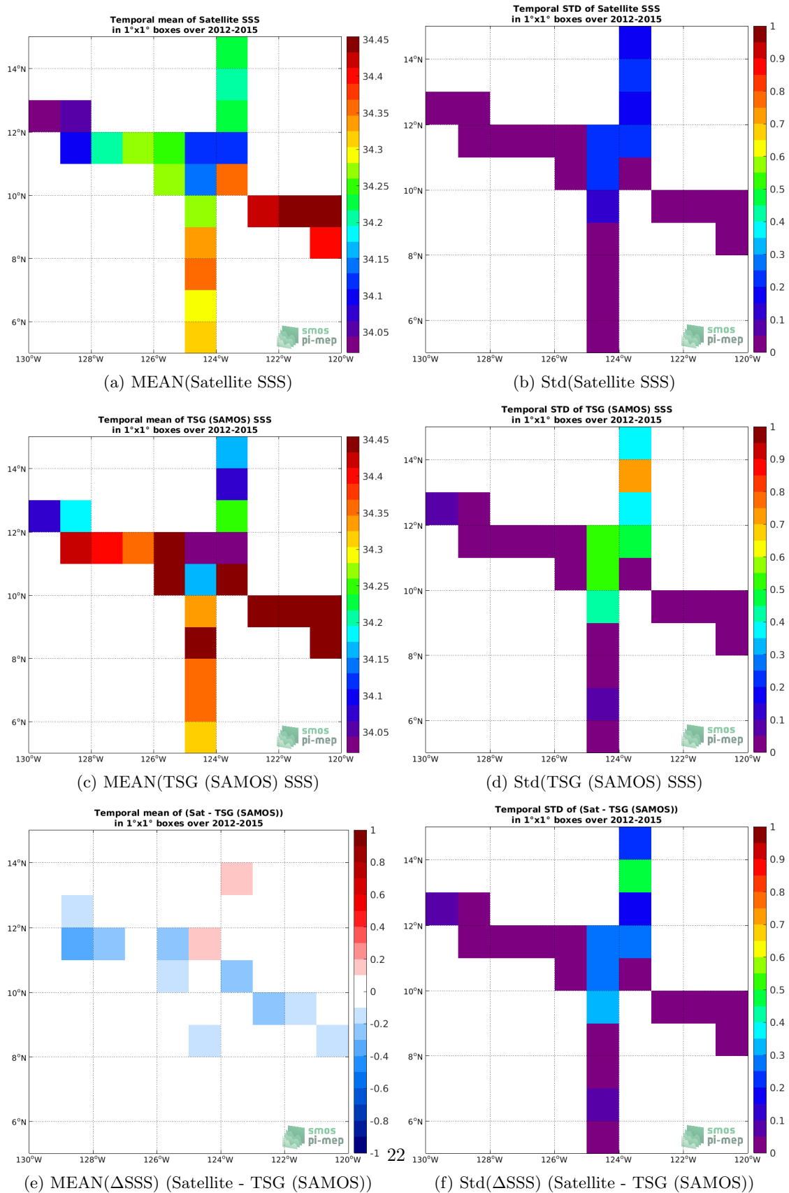
Figure 6: Temporal mean (left) and Std (right) of SSS from Aquarius SSS L4 OI v5 - Weekly (IPRC) (top), TSG (SAMOS) (middle), and of \Delta SSS (Satellite - TSG (SAMOS)). Only match-up pairs are used to generate these maps.
