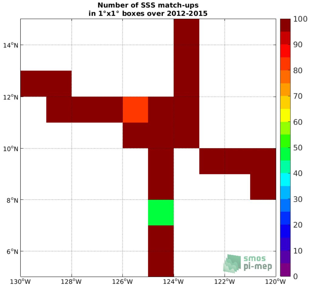
Figure 4: Number of SSS match-ups between TSG (SAMOS) SSS and the Aquarius SSS L4 OI v5 - Weekly (IPRC) SSS product for the SPURS 2 Pi-MEP region over 1°x1° boxes and for the full satellite product period.
