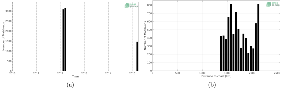
Figure 1: Number of match-ups between TSG (SAMOS) and Aquarius SSS L4 OI v5 - Weekly (IPRC) SSS as a function of time (a) and as function of the distance to coast (b) over the SPURS 2 Pi-MEP region and for the full satellite product period.
