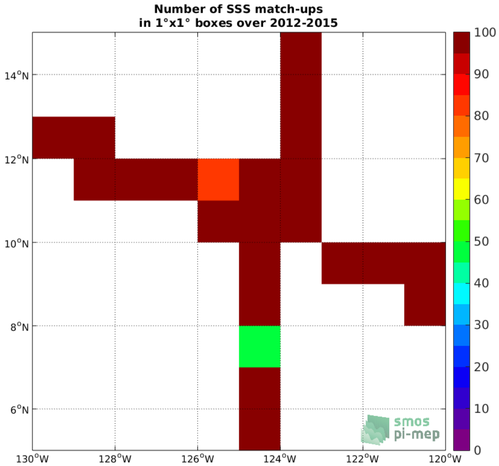
Figure 4: Number of SSS match-ups between TSG-SAMOS SSS and the Aquarius-L4-IPRC-V5-WEEKLY SSS product for the SPURS 2 Pi-MEP region over 1°x1° boxes and for the full satellite product period.
