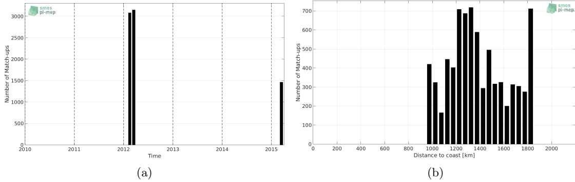
Figure 1: Number of match-ups between TSG-SAMOS and Aquarius-L4-IPRC-V5-WEEKLY SSS as a function of time (a) and as function of the distance to coast (b) over the SPURS 2 Pi-MEP region and for the full satellite product period.
