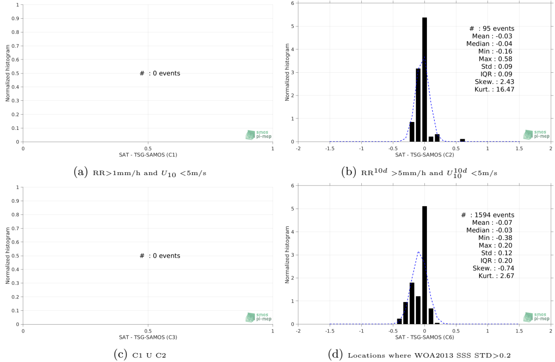
Figure 13: Normalized histogram of \Delta\text{SSS} (Aquarius-L4-IPRC-V5-WEEKLY - TSG-SAMOS) for 6 different subdatasets corresponding to: RR > 1\text{mm/h} and U_{10} < 5\text{m/s} (a), RR^{10d} > 5\text{mm/h} and U_{10}^{10d} < 5\text{m/s} (b), C1 U C2 (c), Locations where WOA2013 SSS STD > 0.2 (d).
