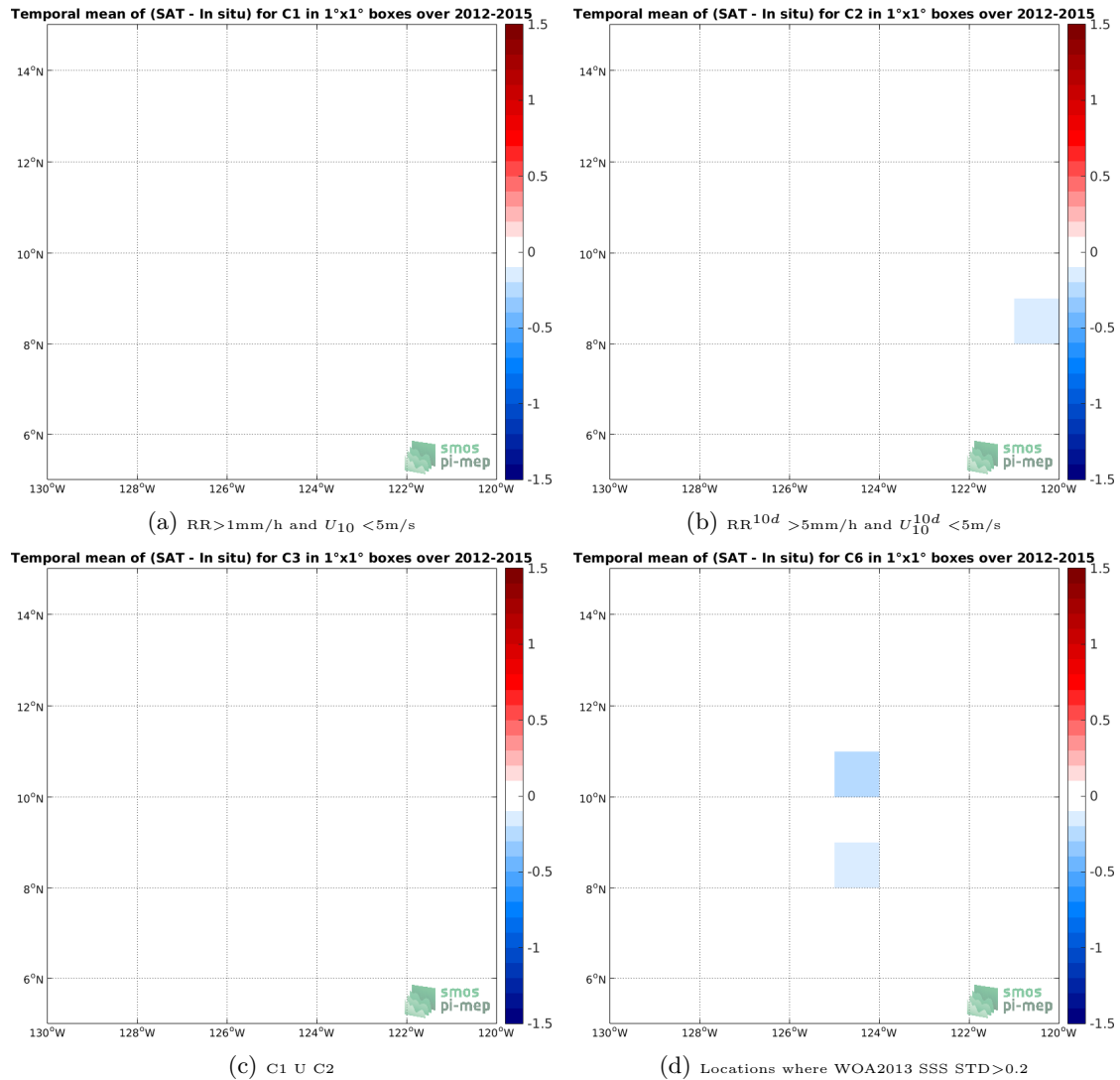
Figure 12: Temporal mean gridded over spatial boxes of size 1^\circ \times 1^\circ of \Delta SSS (Aquarius-L4-IPRC-V5-WEEKLY - TSG-SAMOS) for 4 different subdatasets corresponding to: RR > 1mm/h and U_{10} < 5\text{m/s} (a), RR 10d > 5mm/h and U_{10}^{10d} < 5\text{m/s} (b), C1 U C2 (c), Locations where WOA2013 SSS STD > 0.2 (d).
