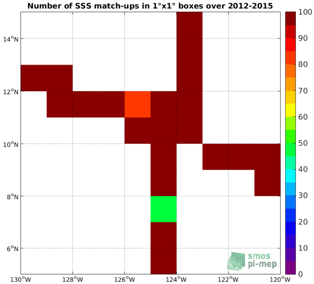
Figure 4: Number of SSS match-ups between TSG-SAMOS SSS and the Aquarius-L4-IPRC-V5-WEEKLY SSS product for the SPURS 2 Pi-MEP region over 1°x1° boxes and for the full satellite product period.
