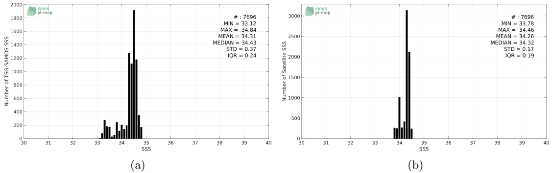
Figure 2: Histograms of SSS from TSG-SAMOS (a) and Aquarius-L4-IPRC-V5-WEEKLY (b) considering all match-up pairs per bins of 0.1 over the SPURS 2 Pi-MEP region and for the full satellite product period.
