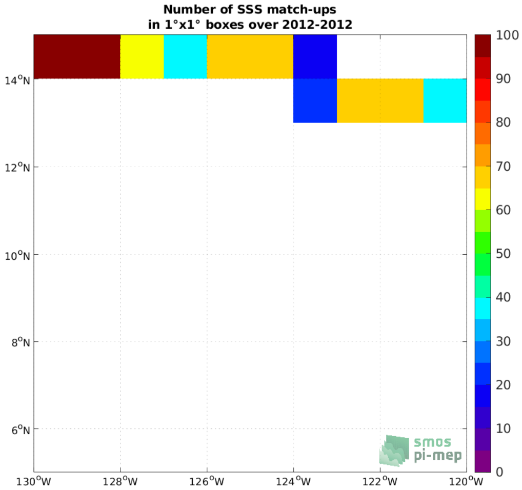
Figure 4: Number of SSS match-ups between TSG (GOSUD-Research-vessel) SSS and the Aquarius SSS L4 OI v5 - Weekly (IPRC) SSS product for the SPURS 2 Pi-MEP region over 1°x1° boxes and for the full satellite product period.
