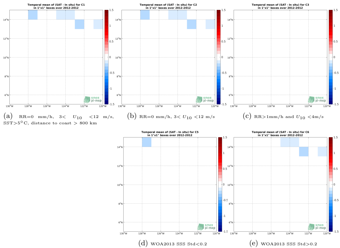
Figure 12: Temporal mean gridded over spatial boxes of size 1^\circ \times 1^\circ of \Delta SSS (Aquarius-L4-IPRC-V5-WEEKLY - TSG-GOSUD-Research-vessel) for 5 different subdatasets corresponding to: RR=0 mm/h, 3 < U_{10} < 12 m/s, SST >5^\circ\text{C} , distance to coast > 800 km (a), RR=0 mm/h, 3 < U_{10} < 12 m/s (b), RR >1 mm/h and U_{10} < 4 m/s (c), WOA2013 SSS Std <0.2 (d), WOA2013 SSS Std >0.2 (e).
