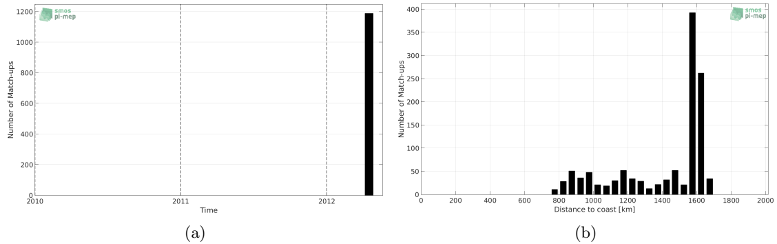
Figure 1: Number of match-ups between TSG-GOSUD-Research-vessel and Aquarius-L4-IPRC-V5-WEEKLY SSS as a function of time (a) and as function of the distance to coast (b) over the SPURS 2 Pi-MEP region and for the full satellite product period.
