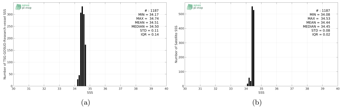
Figure 2: Histograms of SSS from TSG-GOSUD-Research-vessel (a) and Aquarius-L4-IPRC-V5-WEEKLY (b) considering all match-up pairs per bins of 0.1 over the SPURS 2 Pi-MEP region and for the full satellite product period.
