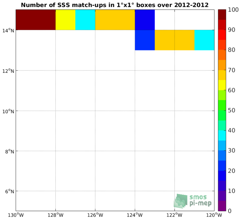
Figure 4: Number of SSS match-ups between TSG-GOSUD-Research-vessel SSS and the Aquarius-L4-IPRC-V5-WEEKLY SSS product for the SPURS 2 Pi-MEP region over 1°x1° boxes and for the full satellite product period.
