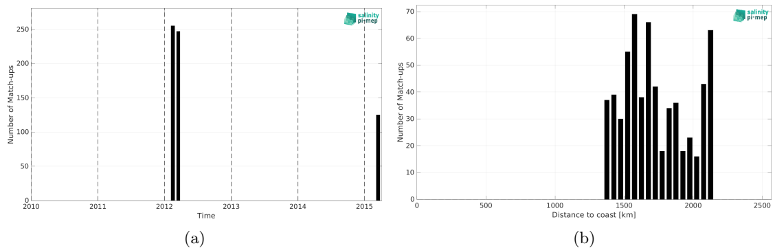
Figure 2: Number of match-ups between TSG (SAMOS) and Aquarius SSS L4 OI v5 - Monthly (IPRC) SSS as a function of time (a) and as function of the distance to coast (b) over the SPURS 2 Pi-MEP region and for the full satellite product period.
