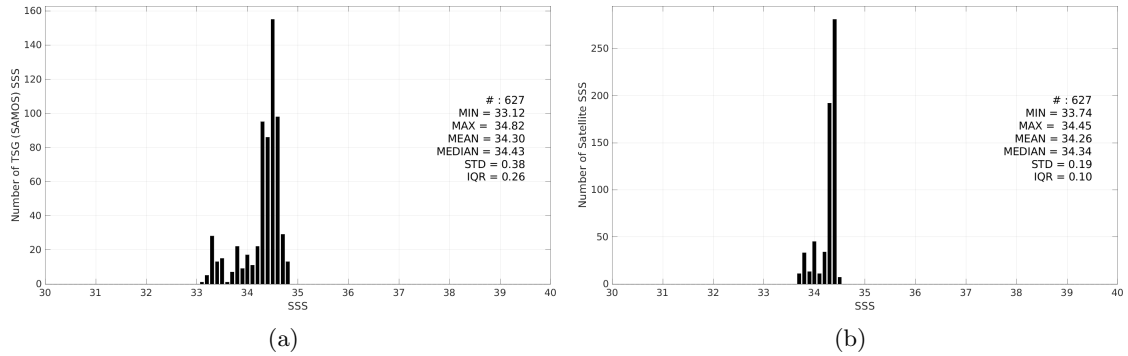
Figure 3: Histograms of SSS from TSG (SAMOS) (a) and Aquarius SSS L4 OI v5 - Monthly (IPRC) (b) considering all match-up pairs per bins of 0.1 over the SPURS 2 Pi-MEP region and for the full satellite product period.
