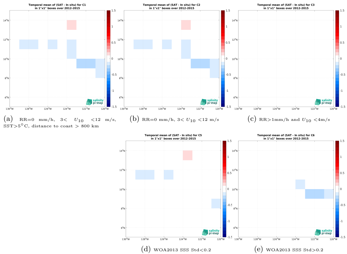
Figure 14: Temporal mean gridded over spatial boxes of size 1^\circ \times 1^\circ of \Delta SSS (Aquarius SSS L4 OI v5 - Monthly (IPRC) - TSG (SAMOS)) for 5 different subdatasets corresponding to:RR=0 mm/h, 3 < U_{10} < 12 m/s, SST>5°C, distance to coast > 800 km (a), RR=0 mm/h, 3 < U_{10} < 12 m/s (b), RR>1mm/h and U_{10} < 4 m/s (c), WOA2013 SSS Std<0.2 (d), WOA2013 SSS Std>0.2 (e).
