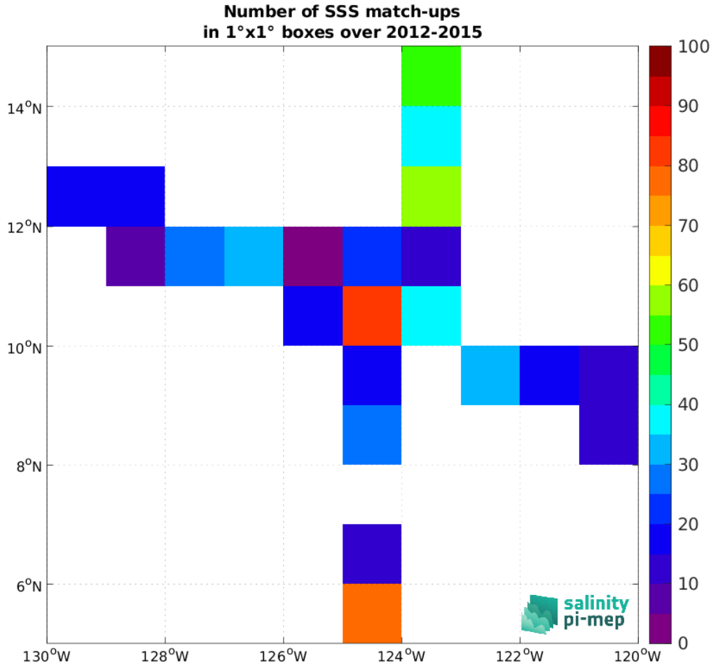
Figure 5: Number of SSS match-ups between TSG (SAMOS) SSS and the Aquarius SSS L4 OI v5 - Monthly (IPRC) SSS product for the SPURS 2 Pi-MEP region over 1^\circ \times 1^\circ boxes and for the full satellite product period.
