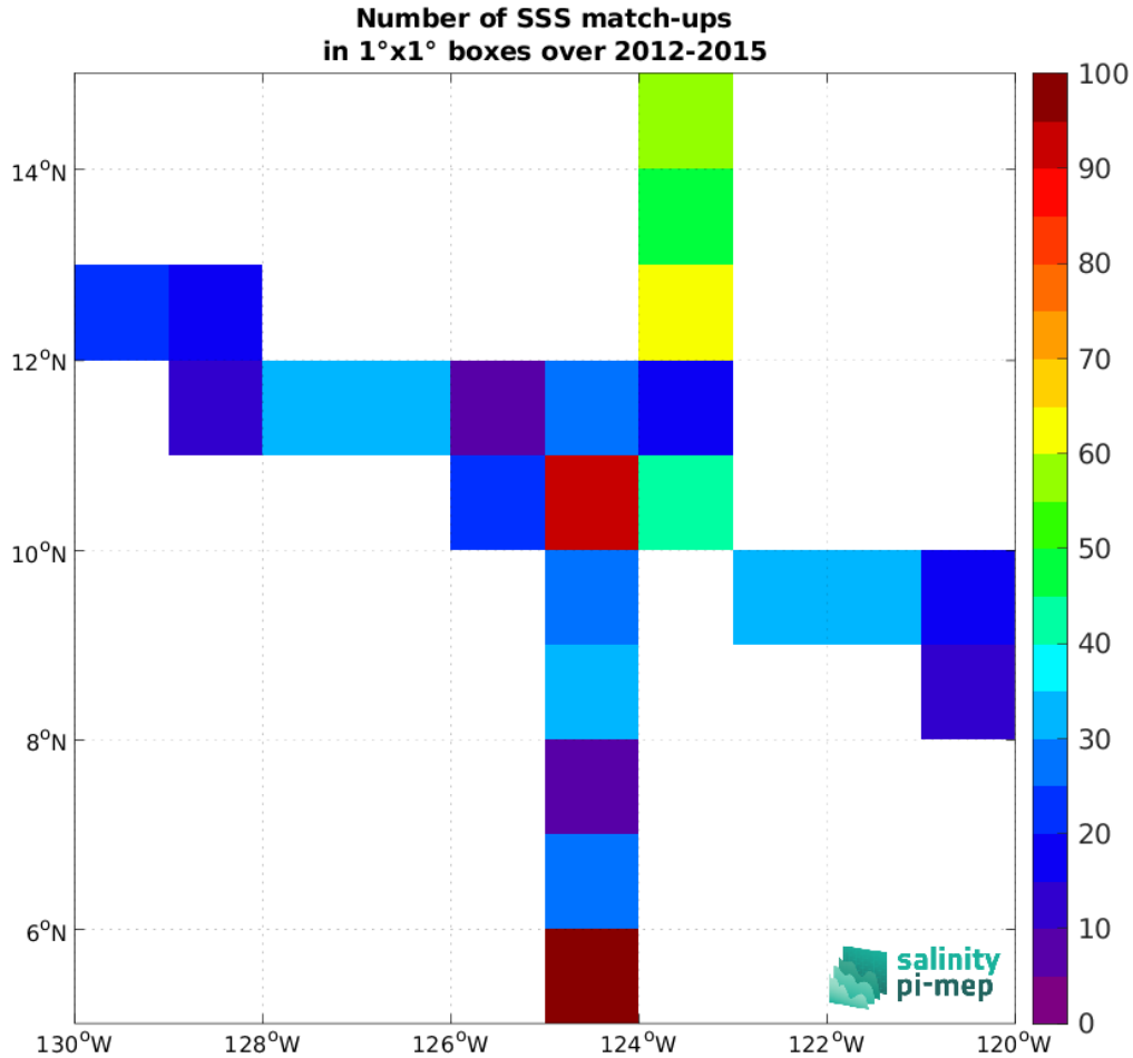
Figure 4: Number of SSS match-ups between TSG (SAMOS) SSS and the Aquarius SSS L4 OI v5 - Monthly (IPRC) SSS product for the SPURS 2 Pi-MEP region over 1^\circ \times 1^\circ boxes and for the full satellite product period.
