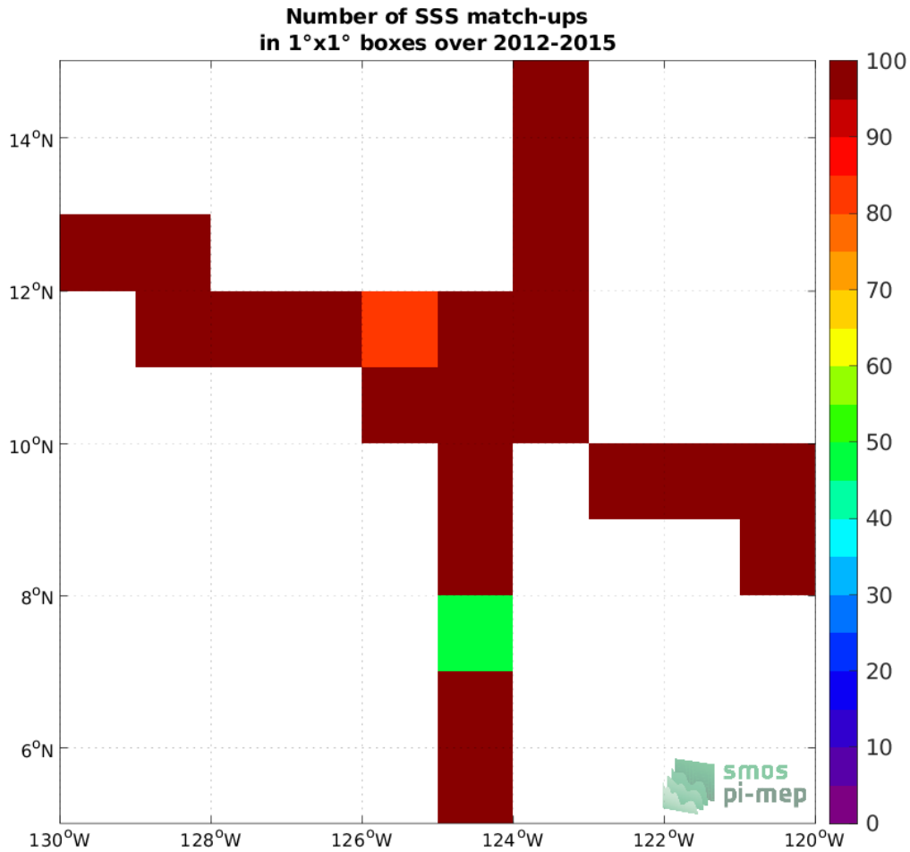
Figure 4: Number of SSS match-ups between TSG (SAMOS) SSS and the Aquarius SSS L4 OI v5 - Monthly (IPRC) SSS product for the SPURS 2 Pi-MEP region over 1°x1° boxes and for the full satellite product period.
