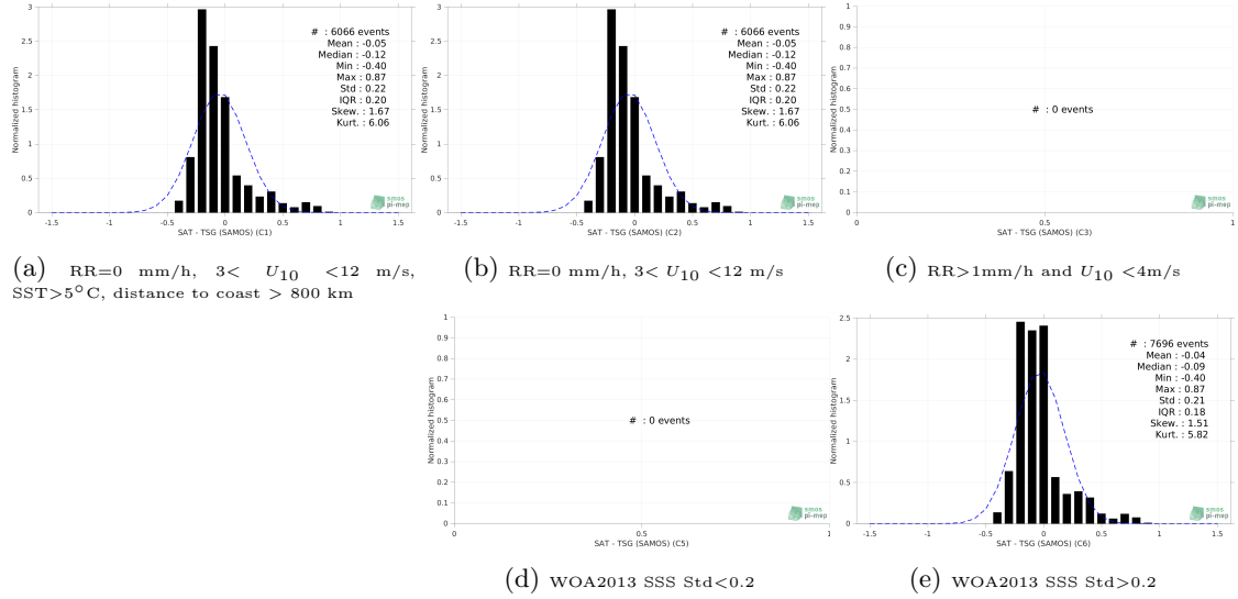
Figure 13: Normalized histogram of \Delta\text{SSS} (Aquarius SSS L4 OI v5 - Monthly (IPRC) - TSG (SAMOS)) for 5 different subdatasets corresponding to: RR=0 mm/h, 3 < U_{10} < 12 m/s, SST > 5^\circ\text{C} , distance to coast > 800 km (a), RR=0 mm/h, 3 < U_{10} < 12 m/s (b), RR > 1\text{mm/h} and U_{10} < 4\text{m/s} (c), WOA2013 SSS \text{Std} < 0.2 (d), WOA2013 SSS \text{Std} > 0.2 (e).
