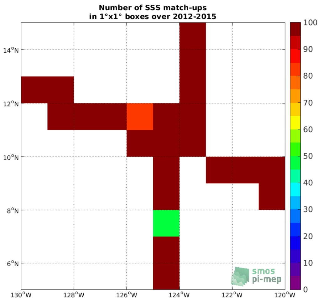
Figure 4: Number of SSS match-ups between TSG-SAMOS SSS and the Aquarius-L4-IPRC-V5-MONTHLY SSS product for the SPURS 2 Pi-MEP region over 1°x1° boxes and for the full satellite product period.
