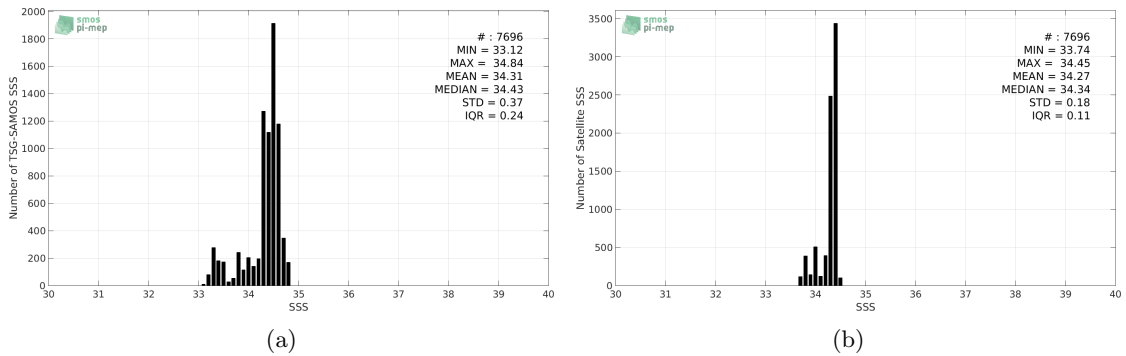
Figure 2: Histograms of SSS from TSG-SAMOS (a) and Aquarius-L4-IPRC-V5-MONTHLY (b) considering all match-up pairs per bins of 0.1 over the SPURS 2 Pi-MEP region and for the full satellite product period.
