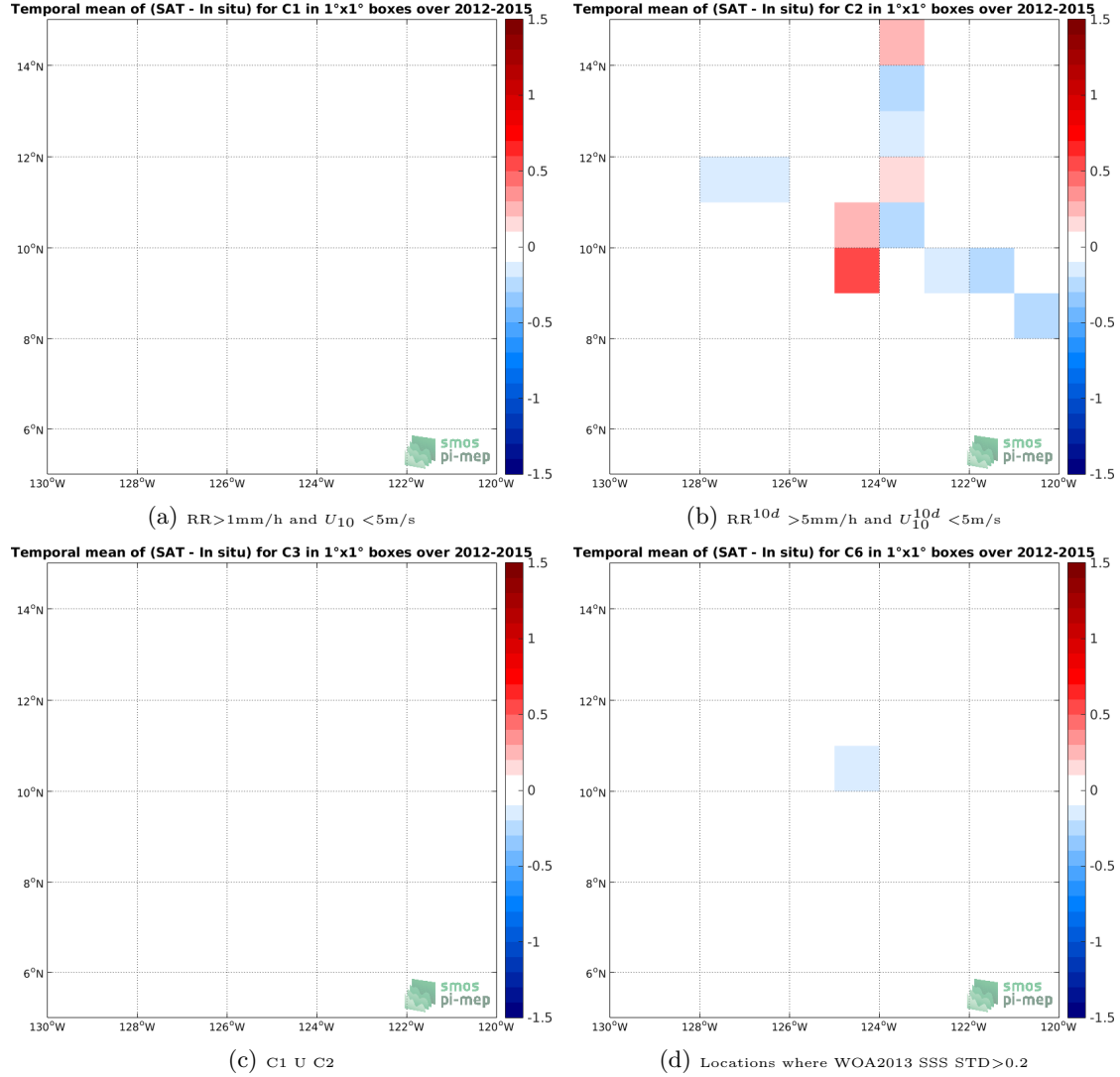
Figure 12: Temporal mean gridded over spatial boxes of size 1^\circ \times 1^\circ of \Delta SSS (Aquarius-L4-IPRC-V5-MONTHLY - TSG-SAMOS) for 4 different subdatasets corresponding to: RR > 1\text{mm/h} and U_{10} < 5\text{m/s} (a), RR^{10d} > 5\text{mm/h} and U_{10}^{10d} < 5\text{m/s} (b), C1 U C2 (c), Locations where WOA2013 SSS STD > 0.2 (d).
