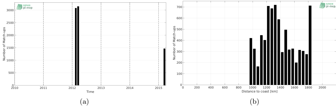
Figure 1: Number of match-ups between TSG-SAMOS and Aquarius-L4-IPRC-V5-MONTHLY SSS as a function of time (a) and as function of the distance to coast (b) over the SPURS 2 Pi-MEP region and for the full satellite product period.
