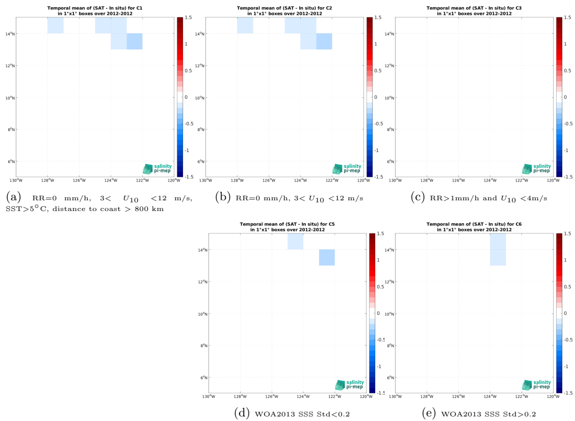
Figure 14: Temporal mean gridded over spatial boxes of size 1^\circ \times 1^\circ of \Delta\text{SSS} (Aquarius SSS L4 OI v5 - Monthly (IPRC) - TSG (GOSUD-Research-vessel)) for 5 different subdatasets corresponding to:RR=0 mm/h, 3 < U_{10} < 12 m/s, SST>5°C, distance to coast > 800 km (a), RR=0 mm/h, 3 < U_{10} < 12 m/s (b), RR>1mm/h and U_{10} < 4 m/s (c), WOA2013 SSS Std<0.2 (d), WOA2013 SSS Std>0.2 (e).
