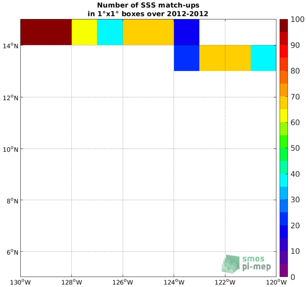
Figure 4: Number of SSS match-ups between TSG (GOSUD-Research-vessel) SSS and the Aquarius SSS L4 OI v5 - Monthly (IPRC) SSS product for the SPURS 2 Pi-MEP region over 1^\circ \times 1^\circ boxes and for the full satellite product period.
