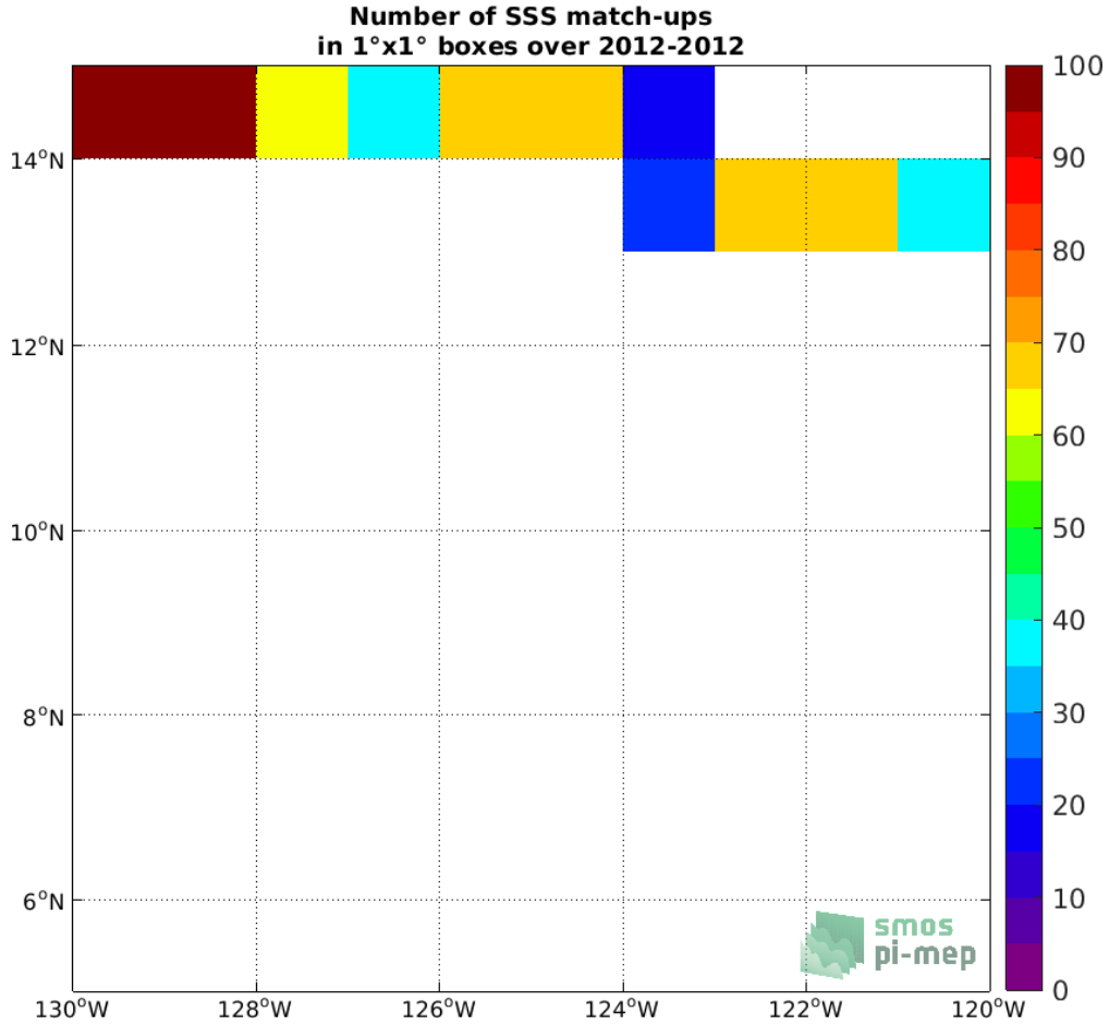
Figure 4: Number of SSS match-ups between TSG (GOSUD-Research-vessel) SSS and the Aquarius SSS L4 OI v5 - Monthly (IPRC) SSS product for the SPURS 2 Pi-MEP region over 1°x1° boxes and for the full satellite product period.
