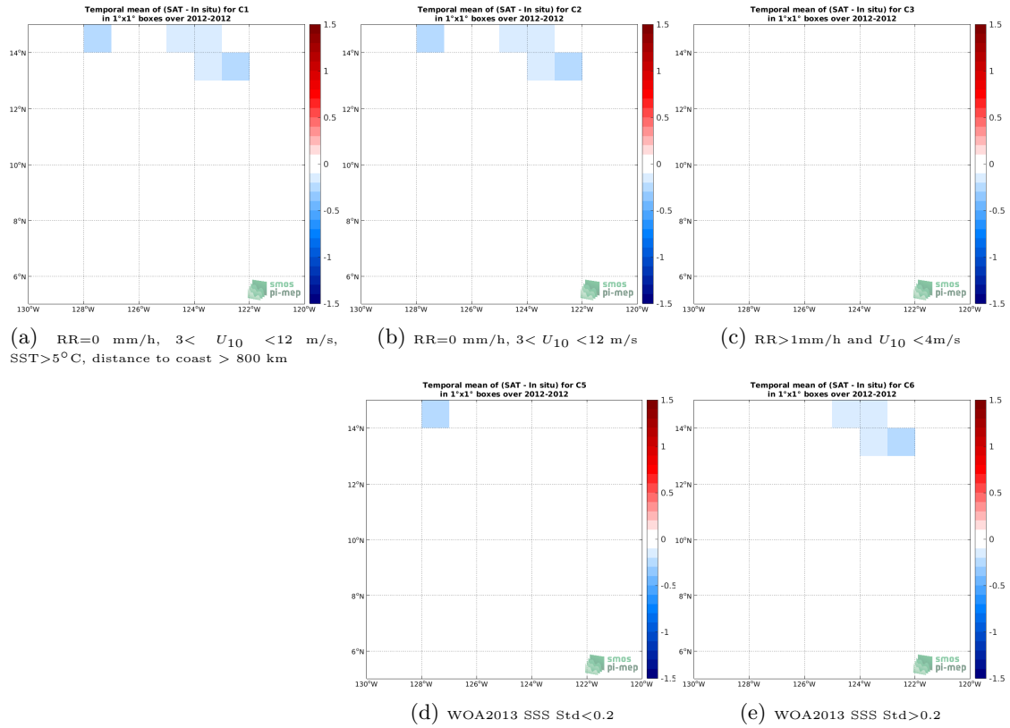
Figure 12: Temporal mean gridded over spatial boxes of size 1^\circ \times 1^\circ of \Delta SSS (Aquarius SSS L4 OI v5 - Monthly (IPRC) - TSG (GOSUD-Research-vessel)) for 5 different subdatasets corresponding to: RR=0 mm/h, 3 < U_{10} < 12 m/s, SST>5°C, distance to coast > 800 km (a), RR=0 mm/h, 3 < U_{10} < 12 m/s (b), RR>1mm/h and U_{10} < 4 m/s (c), WOA2013 SSS Std<0.2 (d), WOA2013 SSS Std>0.2 (e).
