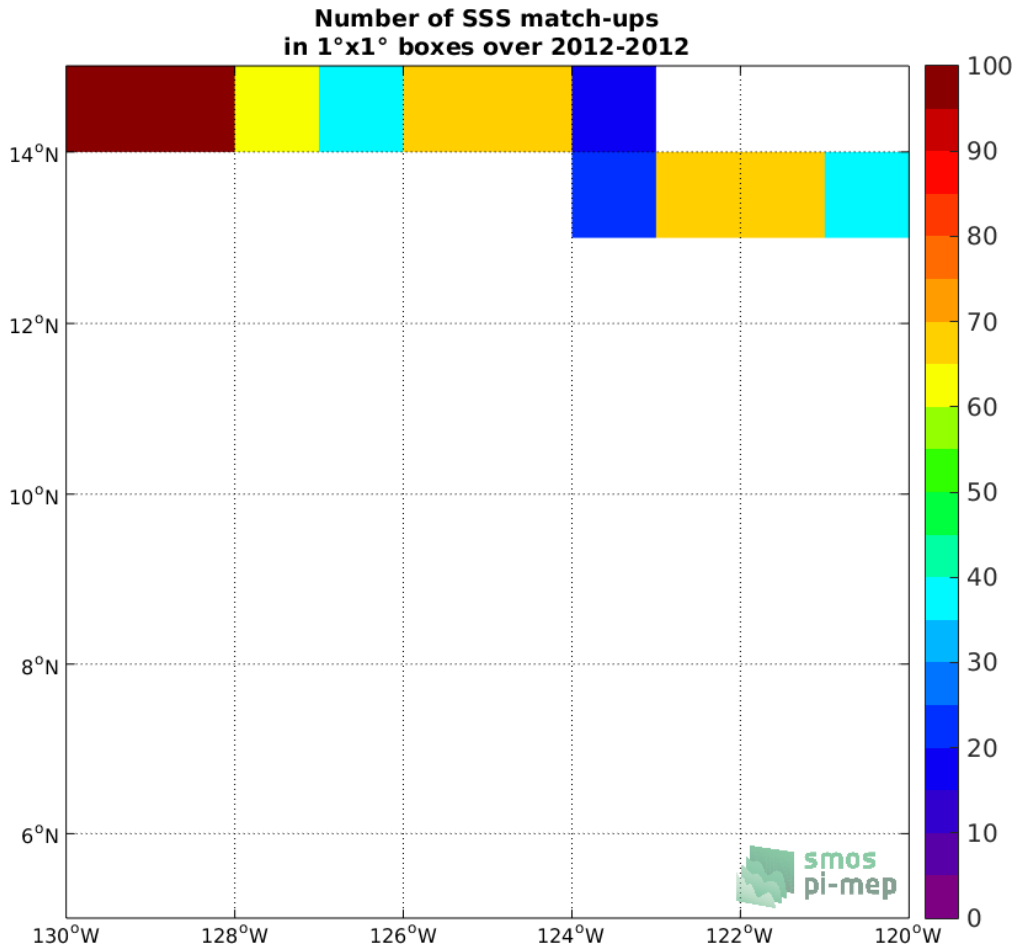
Figure 4: Number of SSS match-ups between TSG-GOSUD-Research-vessel SSS and the Aquarius-L4-IPRC-V5-MONTHLY SSS product for the SPURS 2 Pi-MEP region over 1°x1° boxes and for the full satellite product period.
