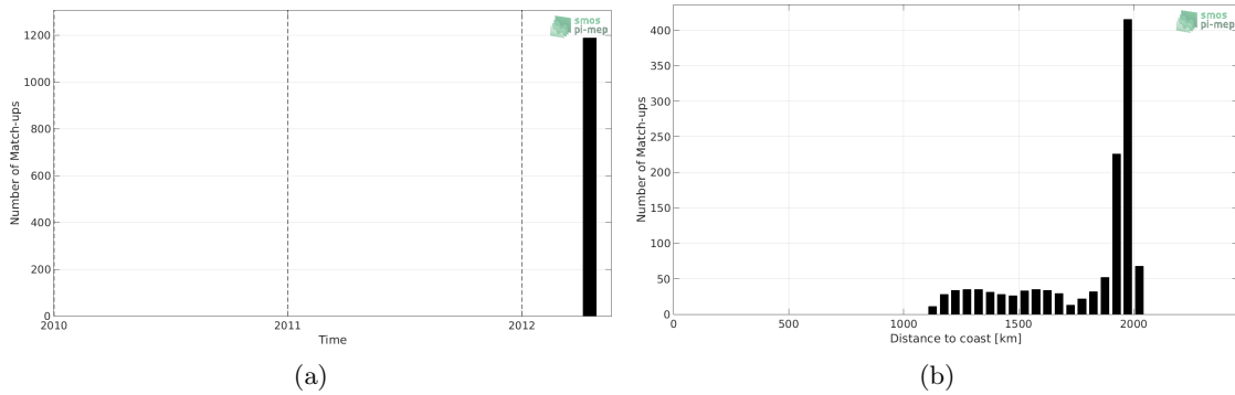
Figure 1: Number of match-ups between TSG-GOSUD-Research-vessel and Aquarius-L4-IPRC-V5-MONTHLY SSS as a function of time (a) and as function of the distance to coast (b) over the SPURS 2 Pi-MEP region and for the full satellite product period.
