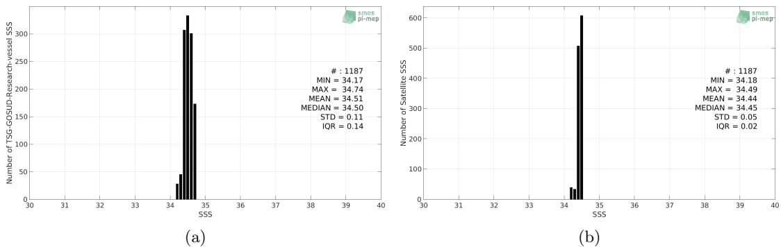
Figure 2: Histograms of SSS from TSG-GOSUD-Research-vessel (a) and Aquarius-L4-IPRC-V5-MONTHLY (b) considering all match-up pairs per bins of 0.1 over the SPURS 2 Pi-MEP region and for the full satellite product period.
