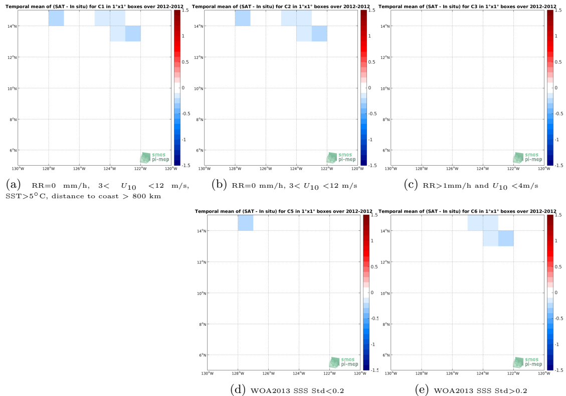
Figure 12: Temporal mean gridded over spatial boxes of size 1^\circ \times 1^\circ of \Delta SSS (Aquarius-L4-IPRC-V5-MONTHLY - TSG-GOSUD-Research-vessel) for 5 different subdatasets corresponding to:RR=0 mm/h, 3 < U_{10} < 12 m/s, SST >5^\circ C, distance to coast > 800 km (a), RR=0 mm/h, 3 < U_{10} < 12 m/s (b), RR >1 mm/h and U_{10} < 4 m/s (c), WOA2013 SSS Std <0.2 (d), WOA2013 SSS Std >0.2 (e).
