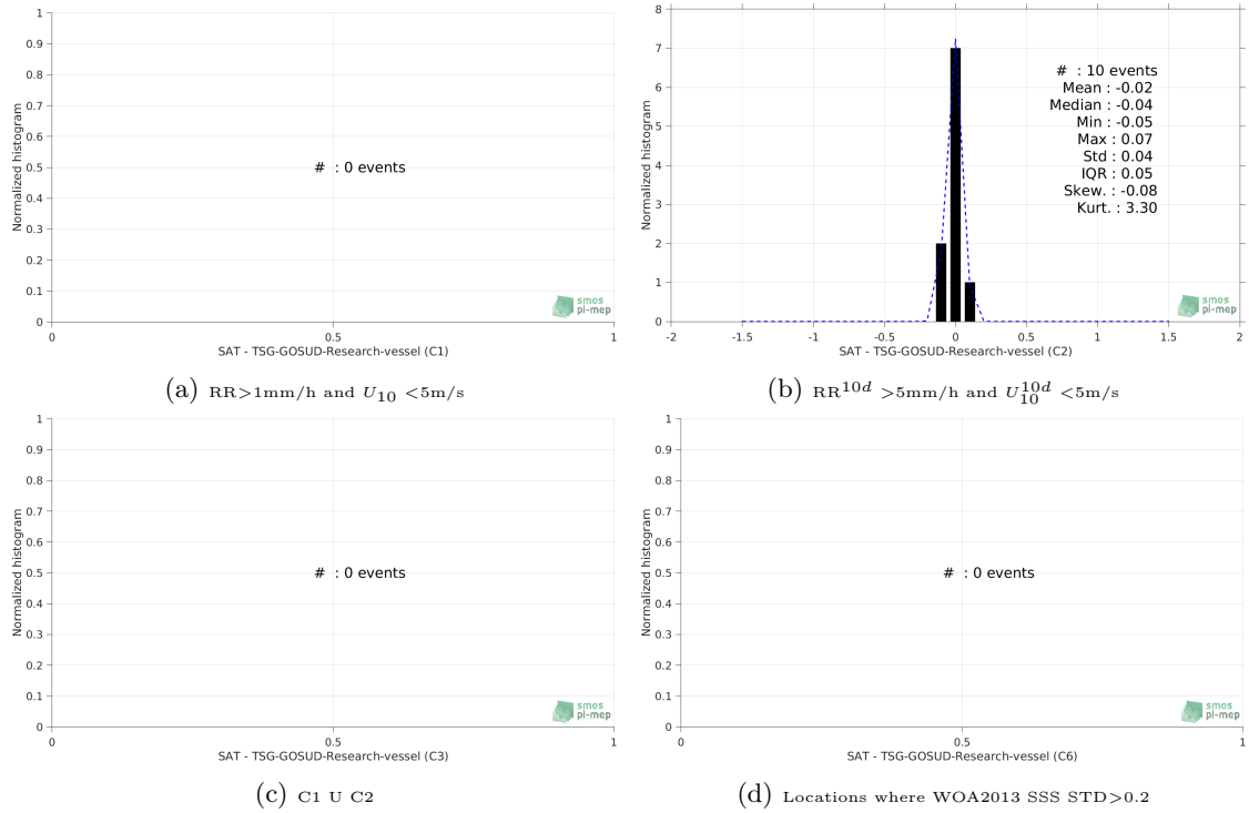
Figure 13: Normalized histogram of \Delta\text{SSS} (Aquarius-L4-IPRC-V5-MONTHLY - TSG-GOSUD-Research-vessel) for 6 different subdatasets corresponding to: RR > 1\text{mm/h} and U_{10} < 5\text{m/s} (a), RR^{10d} > 5\text{mm/h} and U_{10}^{10d} < 5\text{m/s} (b), C1 U C2 (c), Locations where WOA2013 SSS STD > 0.2 (d).
