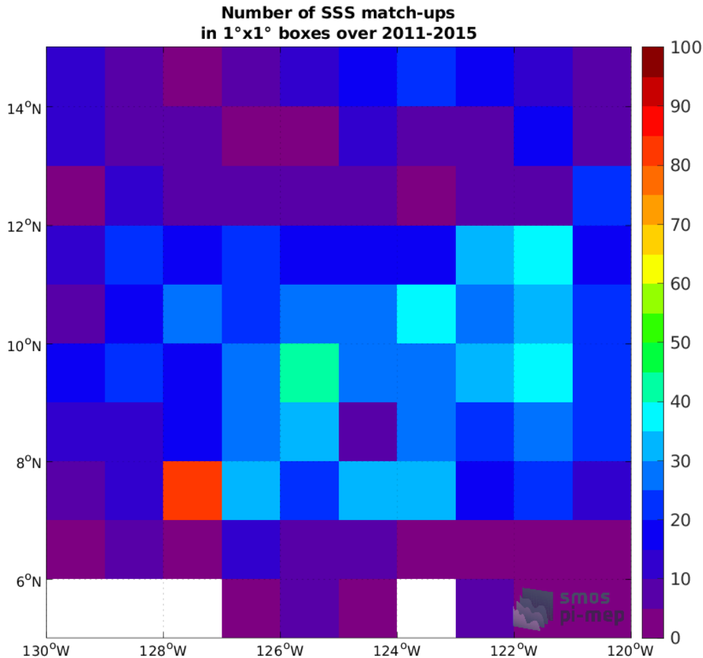
Figure 4: Number of SSS match-ups between Argo SSS and the Aquarius SSS L4 OI v5 - Monthly (IPRC) SSS product for the SPURS 2 Pi-MEP region over 1^\circ \times 1^\circ boxes and for the full satellite product period.
