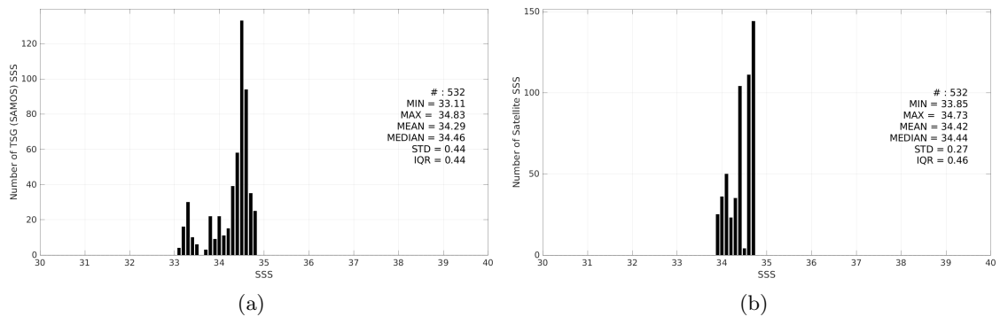
Figure 3: Histograms of SSS from TSG (SAMOS) (a) and Aquarius SSS L3 CAP v5 - 7-Day running (JPL) (b) considering all match-up pairs per bins of 0.1 over the SPURS 2 Pi-MEP region and for the full satellite product period.
