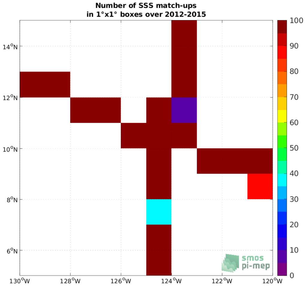
Figure 4: Number of SSS match-ups between TSG (SAMOS) SSS and the Aquarius SSS L3 CAP v5 - 7-Day running (JPL) SSS product for the SPURS 2 Pi-MEP region over 1^\circ \times 1^\circ boxes and for the full satellite product period.
