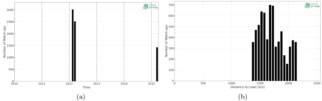
Figure 1: Number of match-ups between TSG-SAMOS and Aquarius-L3-JPL-V5-7DAY-RUNNING SSS as a function of time (a) and as function of the distance to coast (b) over the SPURS 2 Pi-MEP region and for the full satellite product period.
