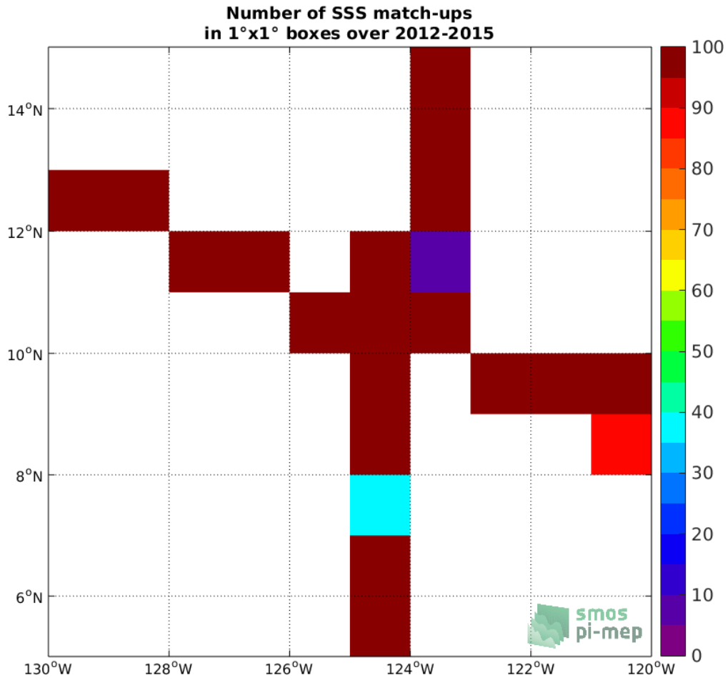
Figure 4: Number of SSS match-ups between TSG-SAMOS SSS and the Aquarius-L3-JPL-V5-7DAY-RUNNING SSS product for the SPURS 2 Pi-MEP region over 1°x1° boxes and for the full satellite product period.
