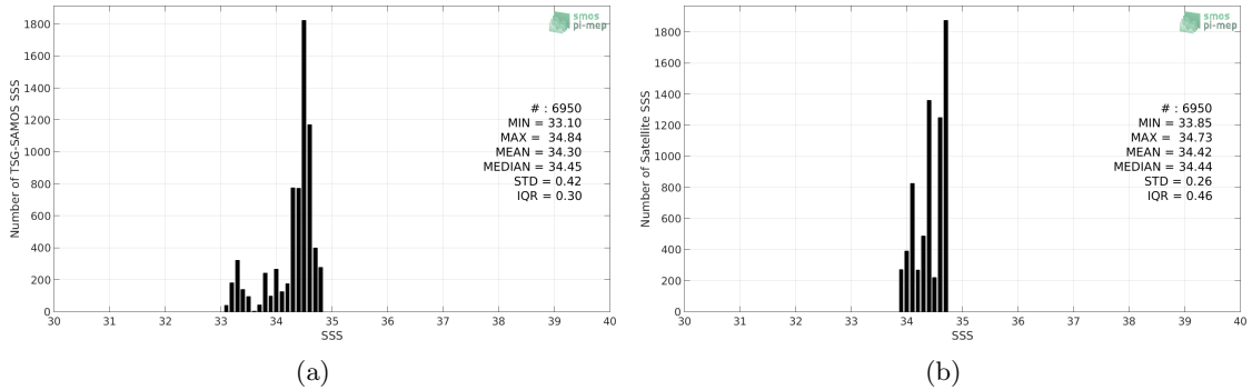
Figure 2: Histograms of SSS from TSG-SAMOS (a) and Aquarius-L3-JPL-V5-7DAY-RUNNING (b) considering all match-up pairs per bins of 0.1 over the SPURS 2 Pi-MEP region and for the full satellite product period.
