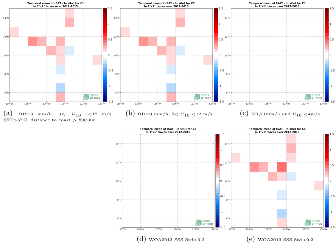
Figure 12: Temporal mean gridded over spatial boxes of size 1^\circ \times 1^\circ of \Delta SSS (Aquarius-L3-JPL-V5-7DAY-RUNNING - TSG-SAMOS) for 5 different subdatasets corresponding to:RR=0 mm/h, 3 < U_{10} < 12 m/s, SST >5^\circ\text{C} , distance to coast > 800 km (a), RR=0 mm/h, 3 < U_{10} < 12 m/s (b), RR >1 mm/h and U_{10} < 4 m/s (c), WOA2013 SSS Std <0.2 (d), WOA2013 SSS Std >0.2 (e).
