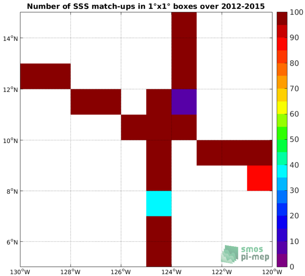
Figure 4: Number of SSS match-ups between TSG-SAMOS SSS and the Aquarius-L3-JPL-V5-7DAY-RUNNING SSS product for the SPURS 2 Pi-MEP region over 1°x1° boxes and for the full satellite product period.
