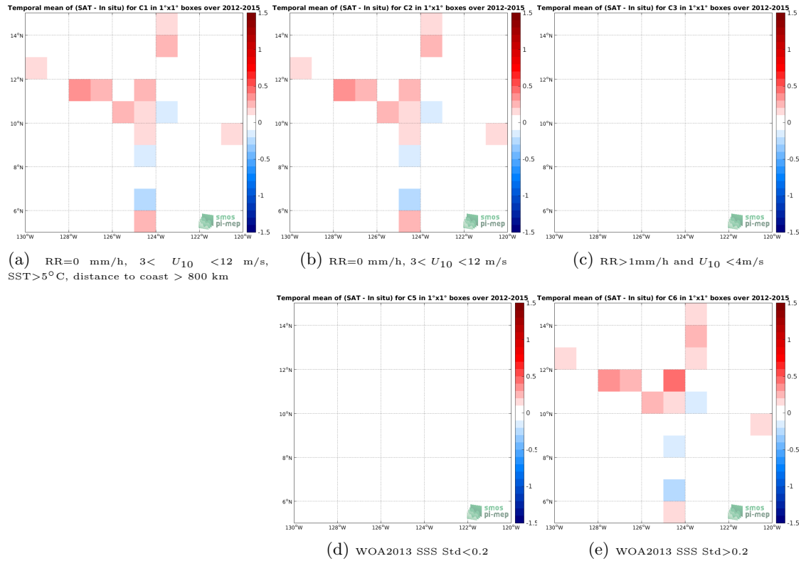
Figure 12: Temporal mean gridded over spatial boxes of size 1^\circ \times 1^\circ of \Delta SSS (Aquarius-L3-JPL-V5-7DAY-RUNNING - TSG-SAMOS) for 5 different subdatasets corresponding to: RR=0 mm/h, 3 < U_{10} < 12 m/s, SST > 5^\circ\text{C} , distance to coast > 800 km (a), RR=0 mm/h, 3 < U_{10} < 12 m/s (b), RR > 1 mm/h and U_{10} < 4 m/s (c), WOA2013 SSS Std <0.2 (d), WOA2013 SSS Std >0.2 (e).
