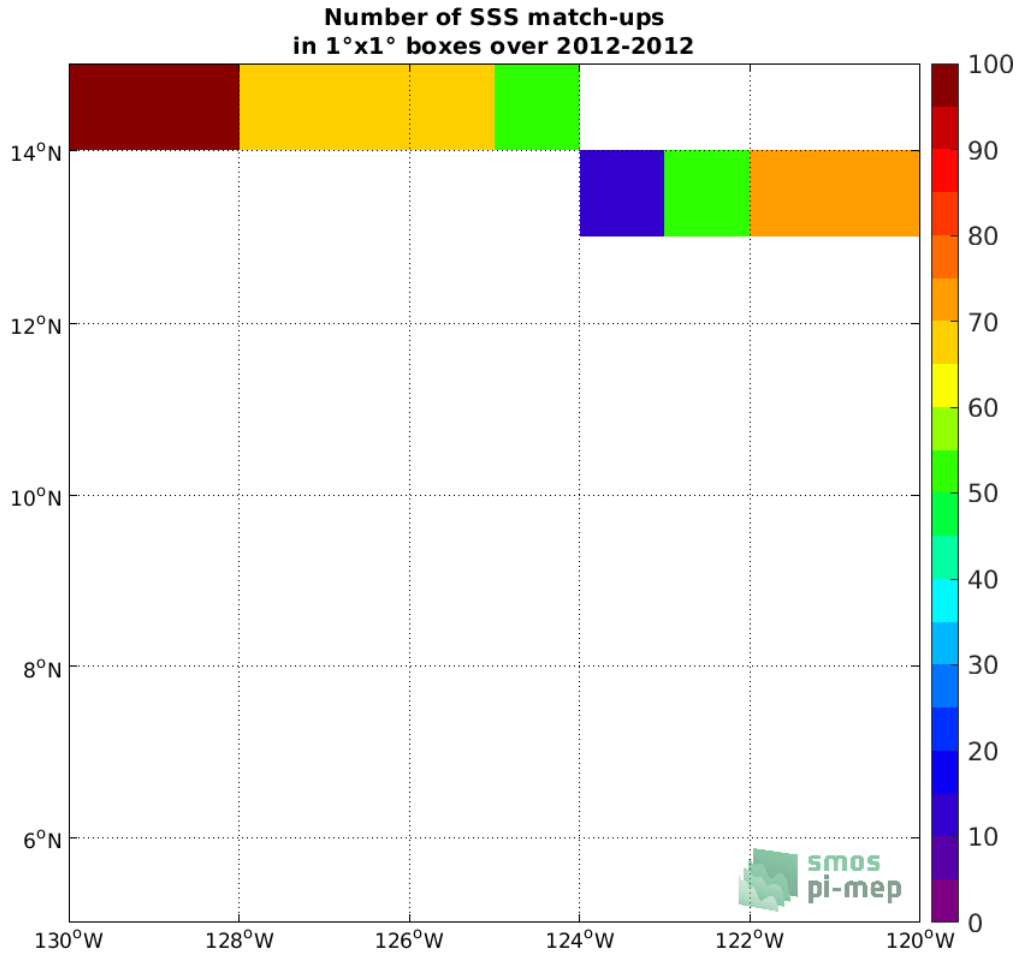
Figure 4: Number of SSS match-ups between TSG (GOSUD-Research-vessel) SSS and the Aquarius SSS L3 CAP v5 - 7-Day running (JPL) SSS product for the SPURS 2 Pi-MEP region over 1°x1° boxes and for the full satellite product period.
