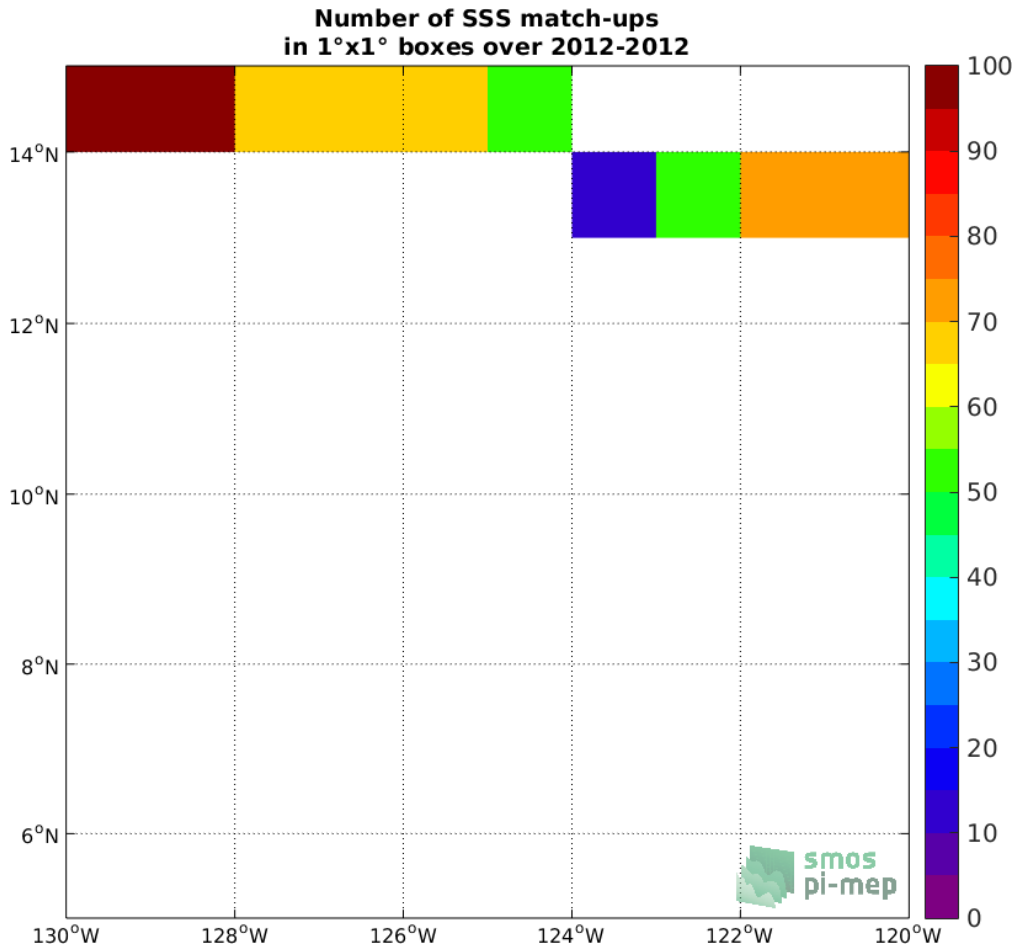
Figure 4: Number of SSS match-ups between TSG-GOSUD-Research-vessel SSS and the Aquarius-L3-JPL-V5-7DAY-RUNNING SSS product for the SPURS 2 Pi-MEP region over 1°x1° boxes and for the full satellite product period.
