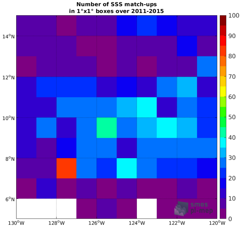
Figure 4: Number of SSS match-ups between Argo SSS and the Aquarius SSS L3 CAP v5 - 7-Day running (JPL) SSS product for the SPURS 2 Pi-MEP region over 1^\circ \times 1^\circ boxes and for the full satellite product period.
