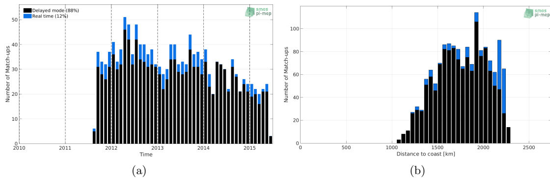
Figure 1: Number of match-ups between Argo and Aquarius-L3-JPL-V5-7DAY-RUNNING SSS as a function of time (a) and as function of the distance to coast (b) over the SPURS 2 Pi-MEP region and for the full satellite product period.
