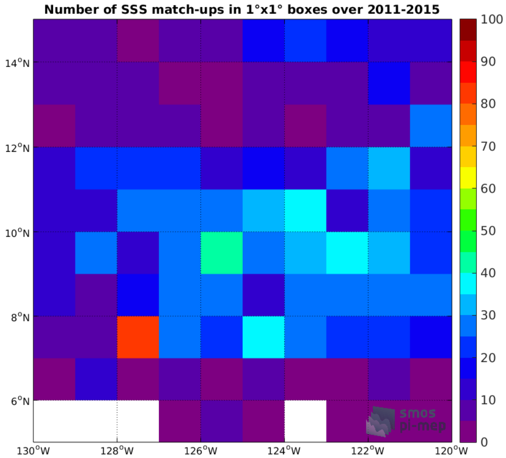
Figure 4: Number of SSS match-ups between Argo SSS and the Aquarius-L3-JPL-V5-7DAY-RUNNING SSS product for the SPURS 2 Pi-MEP region over 1°x1° boxes and for the full satellite product period.
