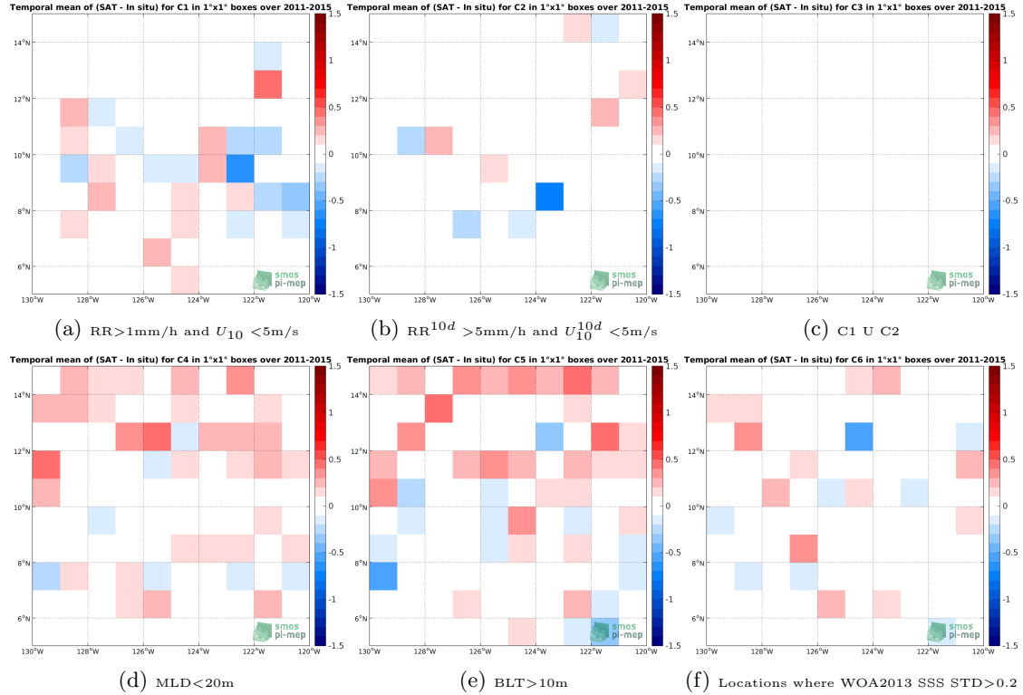
Figure 12: Temporal mean gridded over spatial boxes of size 1^\circ \times 1^\circ of \Delta\text{SSS} (Aquarius-L3-JPL-V5-7DAY-RUNNING - Argo) for 6 different subdatasets corresponding to: \text{RR} > 1\text{mm/h} and U_{10} < 5\text{m/s} (a), \text{RR}^{10d} > 5\text{mm/h} and U_{10}^{10d} < 5\text{m/s} (b), C1 U C2 (c), \text{MLD} < 20\text{m} (d), \text{BLT} > 10\text{m} (e), Locations where WOA2013 SSS STD > 0.2 (f).
