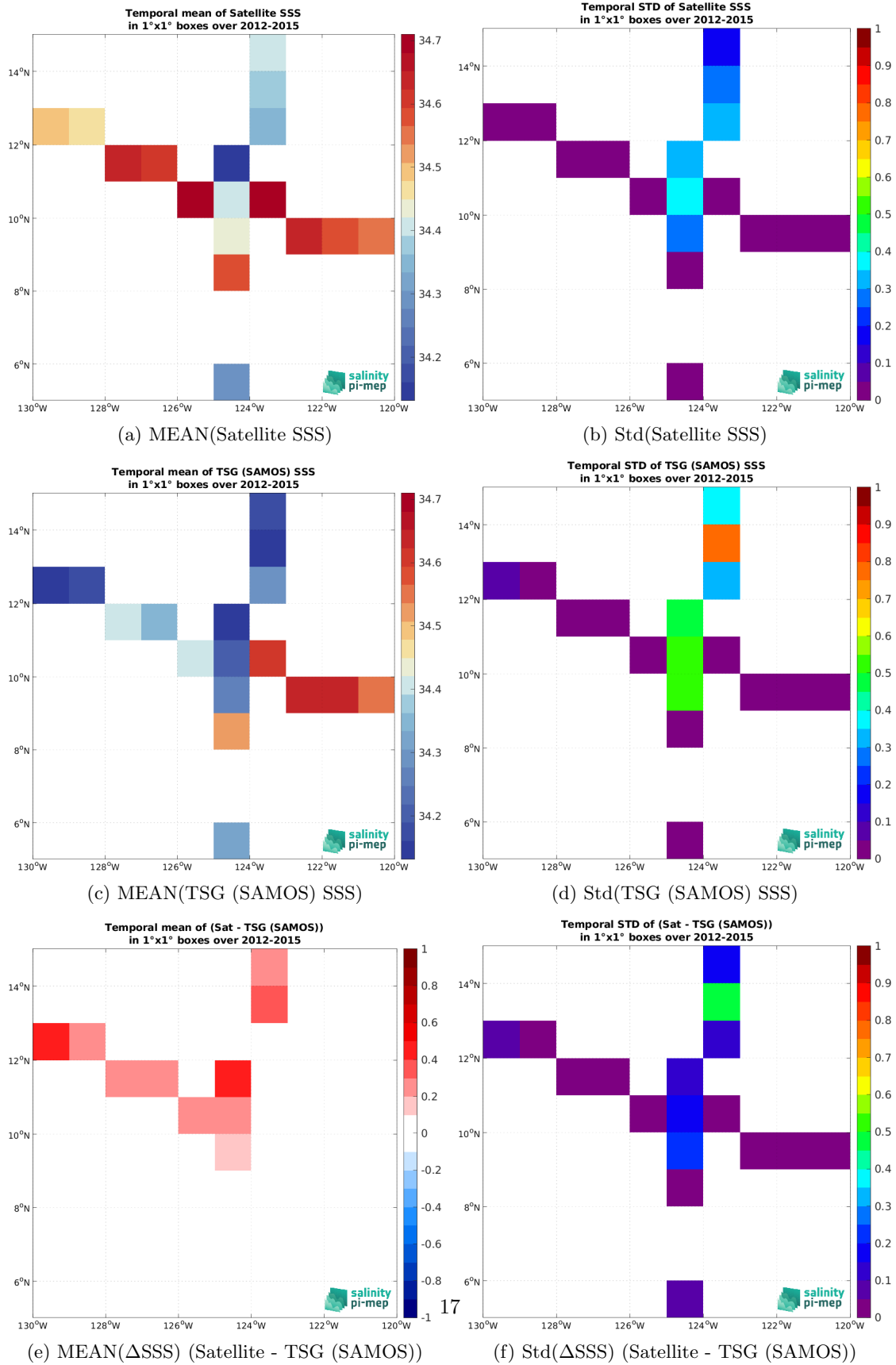
Figure 7: Temporal mean (left) and Std (right) of SSS from Aquarius SSS L3 CAP v5 - Monthly (JPL) (top), TSG (SAMOS) (middle), and of \Delta SSS (Satellite - TSG (SAMOS)). Only match-up pairs are used to generate these maps.
