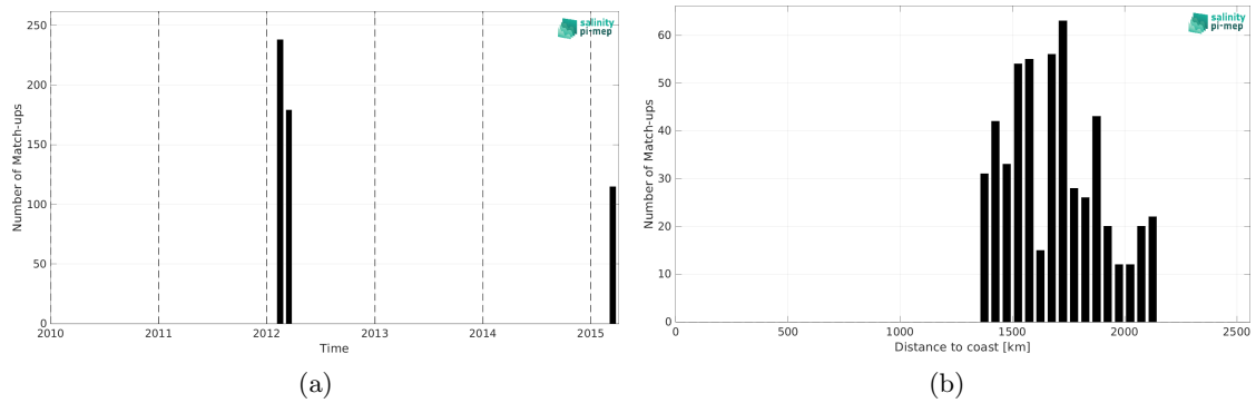
Figure 2: Number of match-ups between TSG (SAMOS) and Aquarius SSS L3 CAP v5 - Monthly (JPL) SSS as a function of time (a) and as function of the distance to coast (b) over the SPURS 2 Pi-MEP region and for the full satellite product period.
