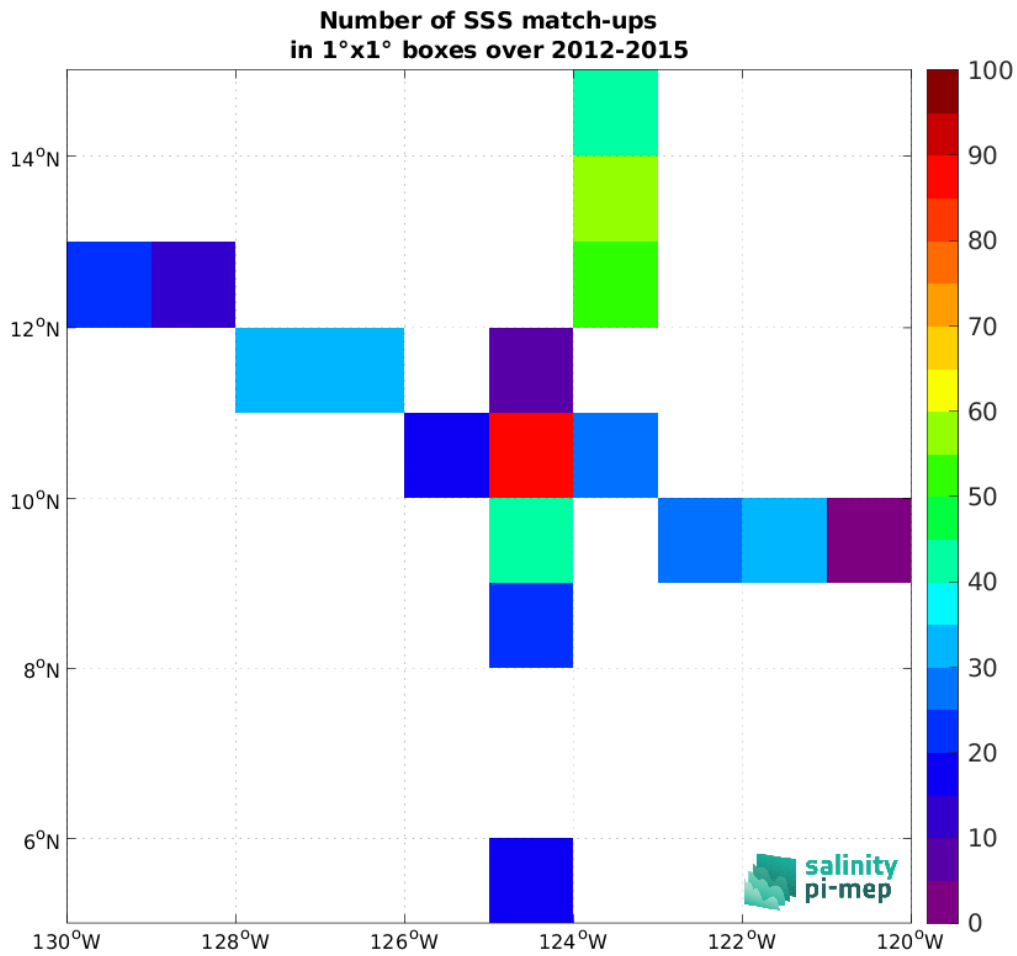
Figure 5: Number of SSS match-ups between TSG (SAMOS) SSS and the Aquarius SSS L3 CAP v5 - Monthly (JPL) SSS product for the SPURS 2 Pi-MEP region over 1^\circ \times 1^\circ boxes and for the full satellite product period.
