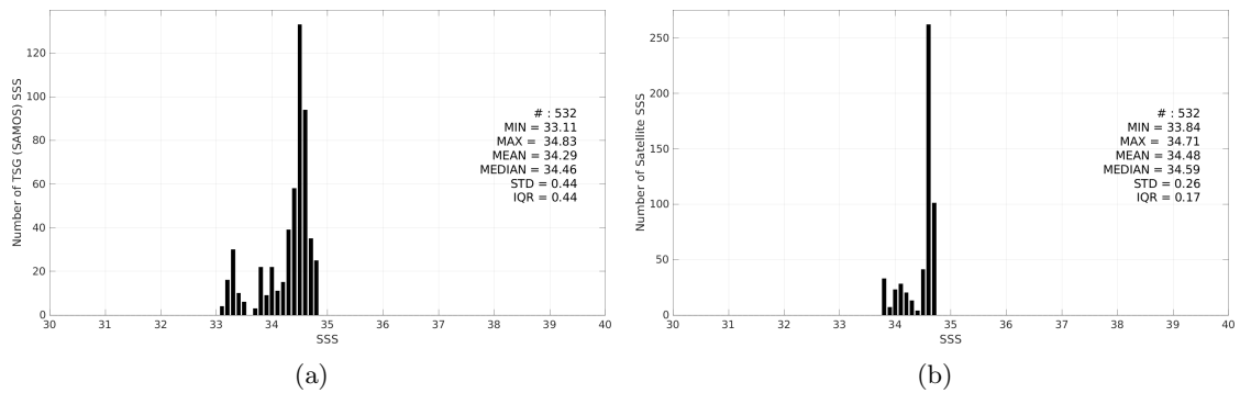
Figure 3: Histograms of SSS from TSG (SAMOS) (a) and Aquarius SSS L3 CAP v5 - Monthly (JPL) (b) considering all match-up pairs per bins of 0.1 over the SPURS 2 Pi-MEP region and for the full satellite product period.
