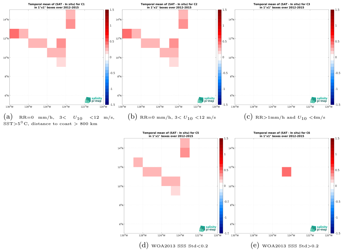
Figure 14: Temporal mean gridded over spatial boxes of size 1^\circ \times 1^\circ of \Delta\text{SSS} (Aquarius SSS L3 CAP v5 - Monthly (JPL) - TSG (SAMOS)) for 5 different subdatasets corresponding to:RR=0 mm/h, 3 < U_{10} < 12 m/s, SST >5^\circ\text{C} , distance to coast > 800 km (a), RR=0 mm/h, 3 < U_{10} < 12 m/s (b), RR >1 mm/h and U_{10} < 4 m/s (c), WOA2013 SSS Std <0.2 (d), WOA2013 SSS Std >0.2 (e).
