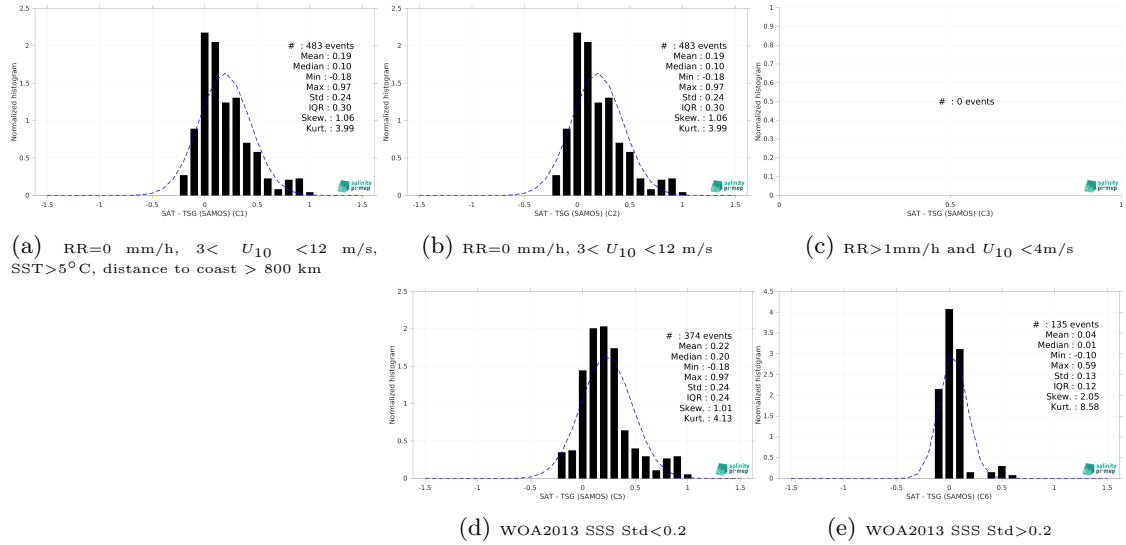
Figure 15: Normalized histogram of \Delta SSS (Aquarius SSS L3 CAP v5 - Monthly (JPL) - TSG (SAMOS)) for 5 different subdatasets corresponding to: RR=0 mm/h, 3 < U_{10} < 12 m/s, SST > 5°C, distance to coast > 800 km (a), RR=0 mm/h, 3 < U_{10} < 12 m/s (b), RR > 1mm/h and U_{10} < 4 m/s (c), WOA2013 SSS Std < 0.2 (d), WOA2013 SSS Std > 0.2 (e).
