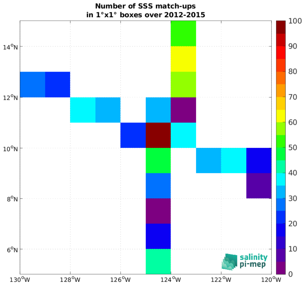
Figure 4: Number of SSS match-ups between TSG (SAMOS) SSS and the Aquarius SSS L3 CAP v5 - Monthly (JPL) SSS product for the SPURS 2 Pi-MEP region over 1^\circ \times 1^\circ boxes and for the full satellite product period.
