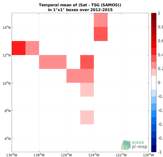
(e) MEAN( \Delta SSS) (Satellite - TSG (SAMOS))
