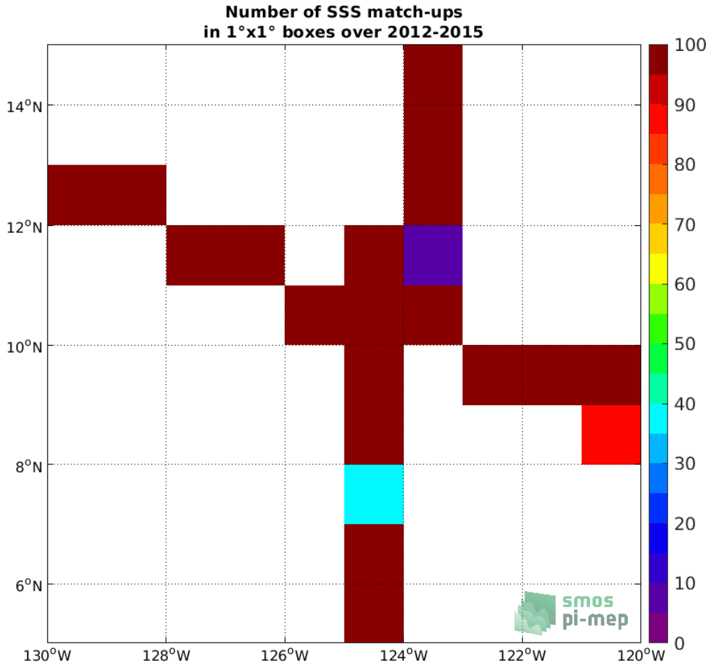
Figure 4: Number of SSS match-ups between TSG (SAMOS) SSS and the Aquarius SSS L3 CAP v5 - Monthly (JPL) SSS product for the SPURS 2 Pi-MEP region over 1°x1° boxes and for the full satellite product period.
