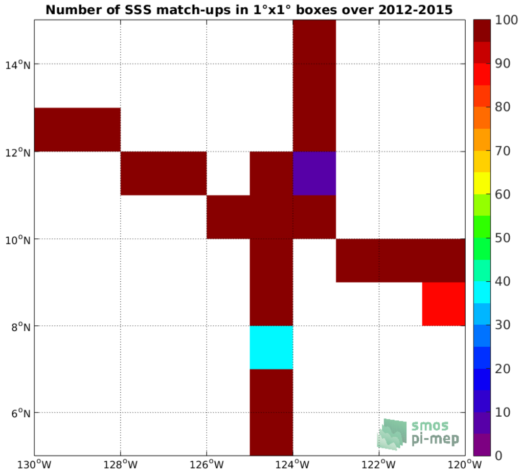
Figure 4: Number of SSS match-ups between TSG-SAMOS SSS and the Aquarius-L3-JPL-V5-MONTHLY SSS product for the SPURS 2 Pi-MEP region over 1°x1° boxes and for the full satellite product period.
