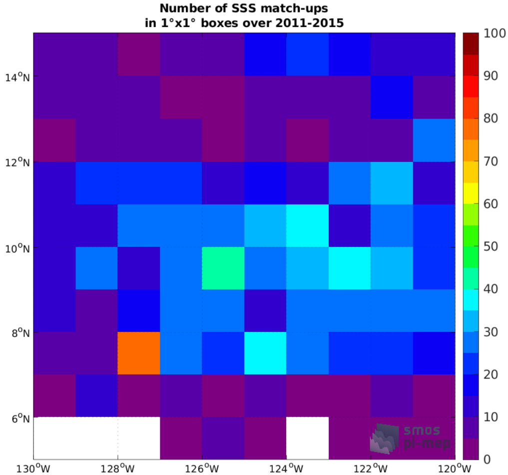
Figure 4: Number of SSS match-ups between Argo SSS and the Aquarius SSS L3 CAP v5 - Monthly (JPL) SSS product for the SPURS 2 Pi-MEP region over 1^\circ \times 1^\circ boxes and for the full satellite product period.
